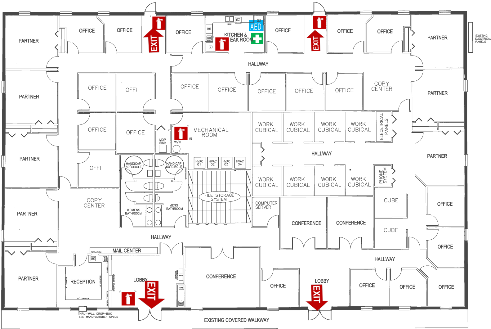
PROPOSED FLOOR LAYOUT
