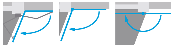
Motorization with arm up to 110°
