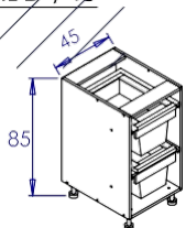
Bambo Drawer-Unit * 2 Drawers(X)×15.1 cm.
