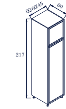
Tail-Unit 2 * 1 Front (X) ×37.5 cm. * 1 Front (X) ×169.5 cm. * 2 Shelves
