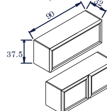
HOOD-Unit * 1 Front 90x37.5 Or * 2 Fronts 45x37.5 cm.
