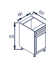
LOWER 1 Drawe r-Unit * 1 Drawe r 60 ×15.1 cm. * 1 Front 60×59.8 cm. * 1 Shelf
