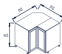
LOWER Corner-Unit * 2 Fronts 35×75 cm. * Witho ut Shelf ( BLC2-92-SH)
