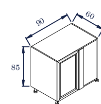
LOWER Corner-Unit * 1 Front 45×75 cm. * 1 Shelf
