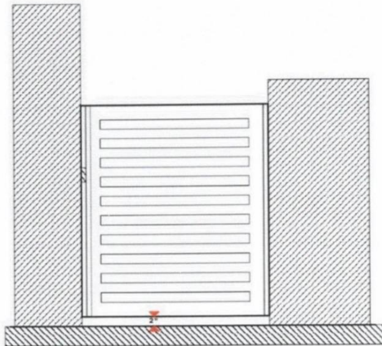
FRONT VIEW
