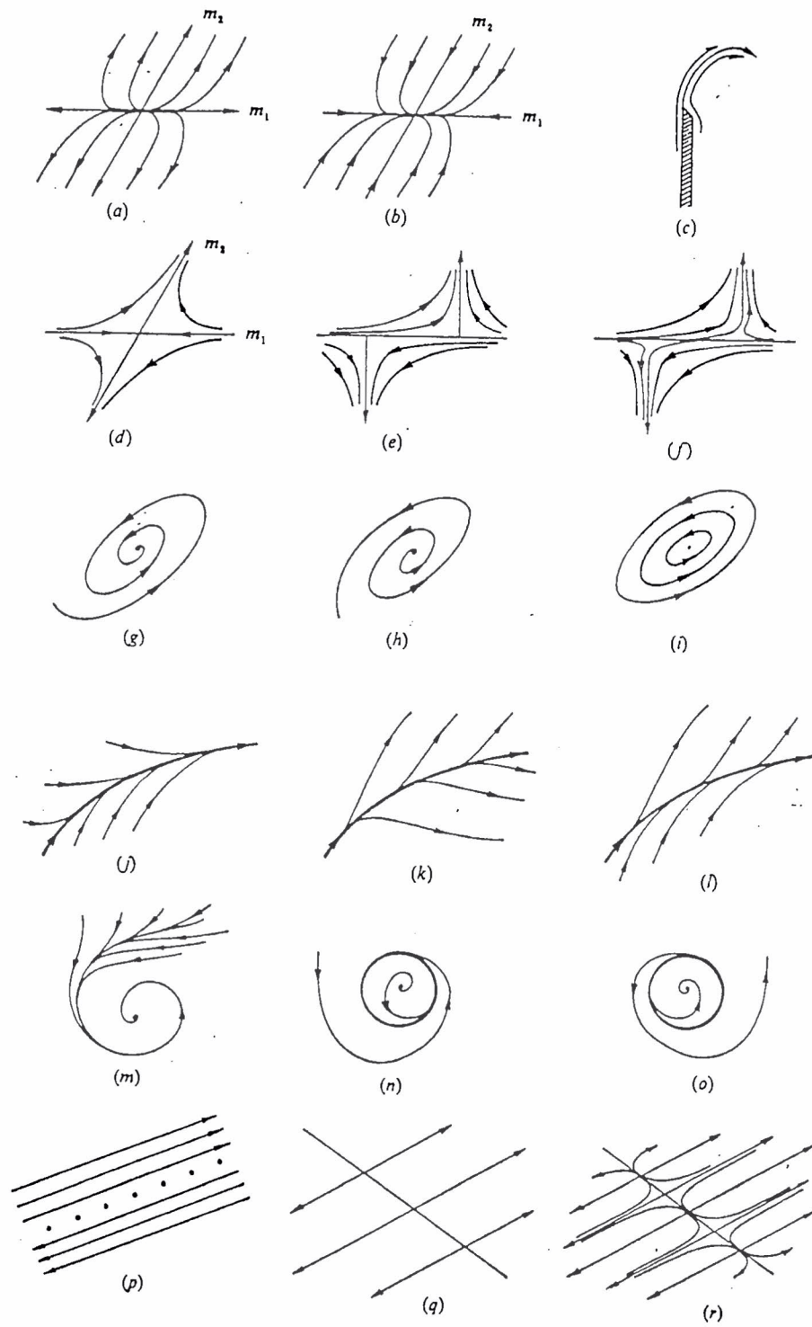
Figure 1.4: Examples of possible critical point topologies (Perry & Steiner, 1987, Part I)
