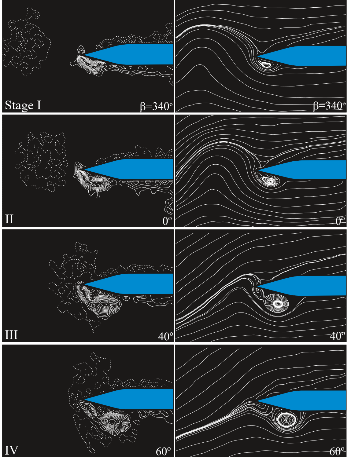
Figure 6.13: Instantaneous vorticity distributions and streamline patterns in the laboratory reference frame depicting the stages of tip vortex development for a stationary leading-edge with an incident clockwise vortex. |\omega_{\min}| = 5 \text{ sec}^{-1} and \Delta\omega = 5 \text{ sec}^{-1} . \text{Re} = 6,250 .
