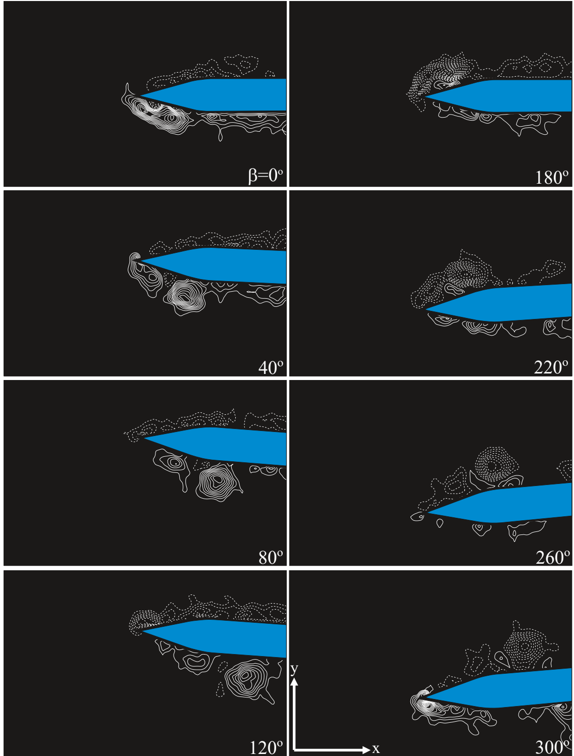
Figure 5.2: Instantaneous vorticity distributions showing symmetric vortex development for an oscillating leading-edge without an incident vortex. |\omega_{\min}| = 5 \text{ sec}^{-1} and \Delta\omega = 5 \text{ sec}^{-1} . \text{Re} = 6,250 .
