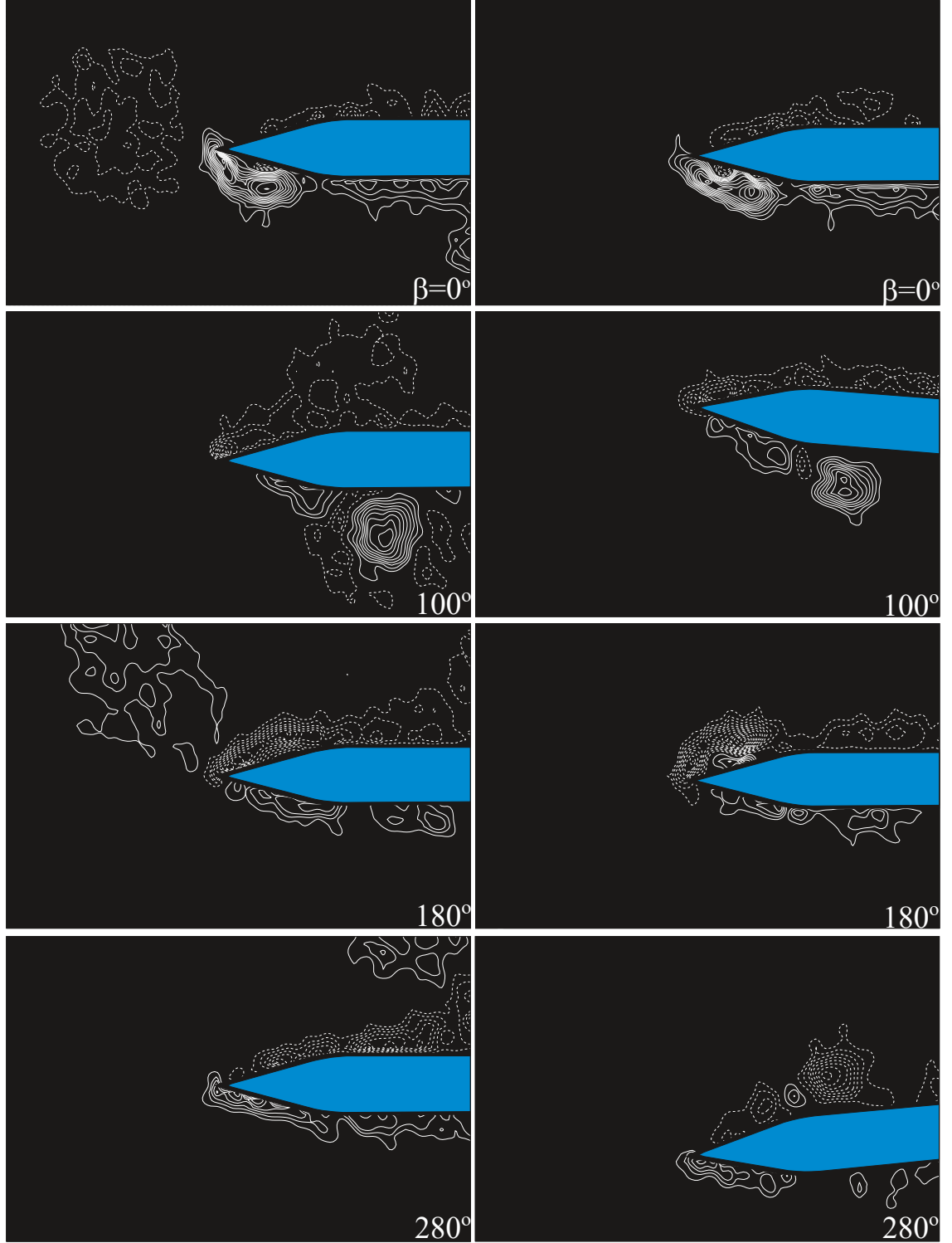
Figure 6.2: Comparison of the vorticity distributions for an incident vortex impinging a stationary leading-edge (left column) with those of a leading-edge oscillating without an incident vortex (right column). |\omega_{\min}| = 5 \text{ sec}^{-1} ; \Delta\omega = 5 \text{ sec}^{-1} . \text{Re}=6,250 .
