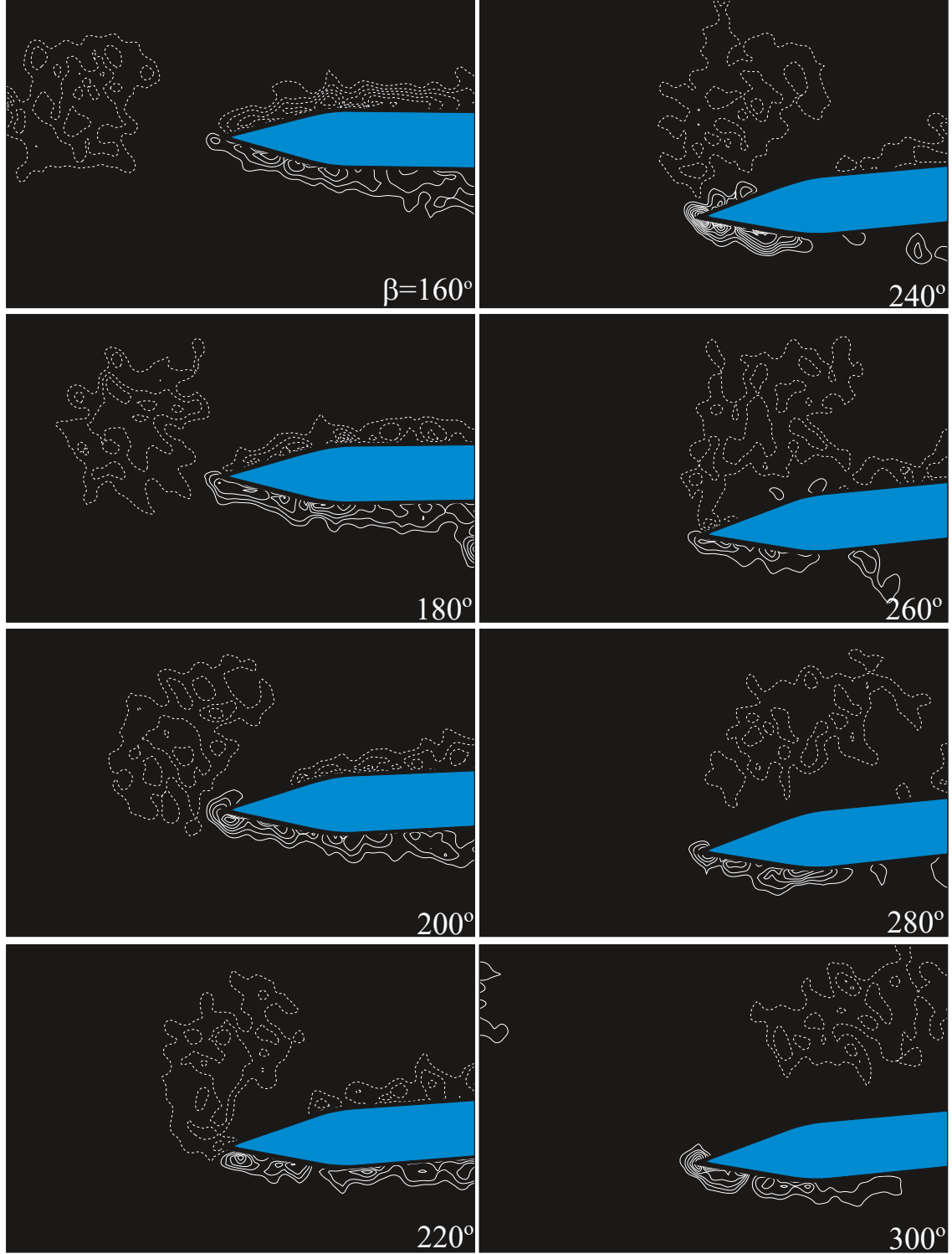
Figure 5.15: Instantaneous vorticity distributions for an oscillating leading-edge at \phi = 180^\circ with respect to an incident clockwise vortex. |\omega_{\min}| = 5 \text{ sec}^{-1} ; \Delta\omega = 5 \text{ sec}^{-1} . \text{Re} = 6,250 .
