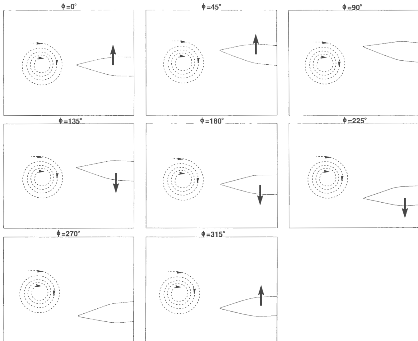
Figure 2.2: Schematic of Representative Phase Angles for an Oscillating Leading-Edge
