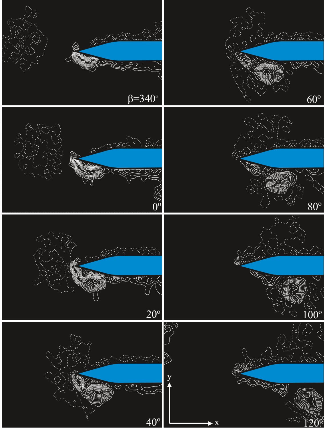
Figure 4.1 : Instantaneous vorticity distributions for a stationary leading-edge at \alpha=0^\circ with an incident clockwise vortex. Re= 6,250 . Contours of negative vorticity, corresponding to clockwise rotation, are denoted as dashed lines, while positive vorticity is represented by solid lines. Minimum and incremental contour levels are |\omega_{min}|= 5 \text{ sec}^{-1} and \Delta\omega= 5 \text{ sec}^{-1}
