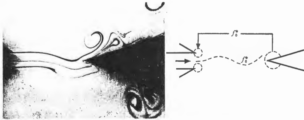
a) Self-sustained oscillations of a jet impinging upon a stationary edge.
