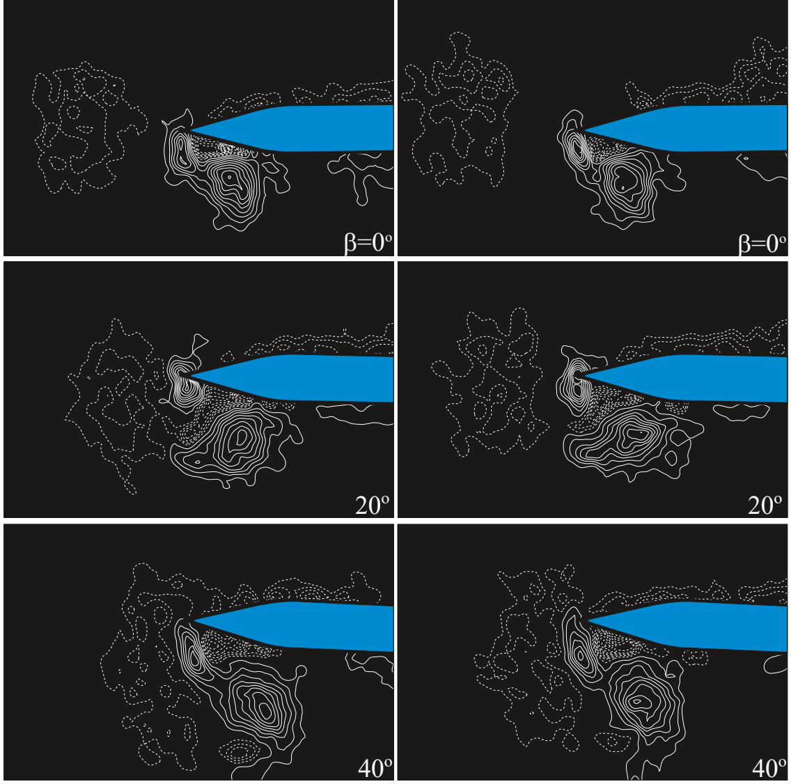
Figure 5.9: Comparison of the instantaneous vorticity distributions from two different cycles for an oscillating leading-edge at \phi = 0^\circ with respect to an incident clockwise vortex. |\omega_{\min}| = 5 \text{ sec}^{-1} ; negative contours, \Delta\omega = 5 \text{ sec}^{-1} ; positive contours, \Delta\omega = 10 \text{ sec}^{-1} . \text{Re} = 6,250 .
