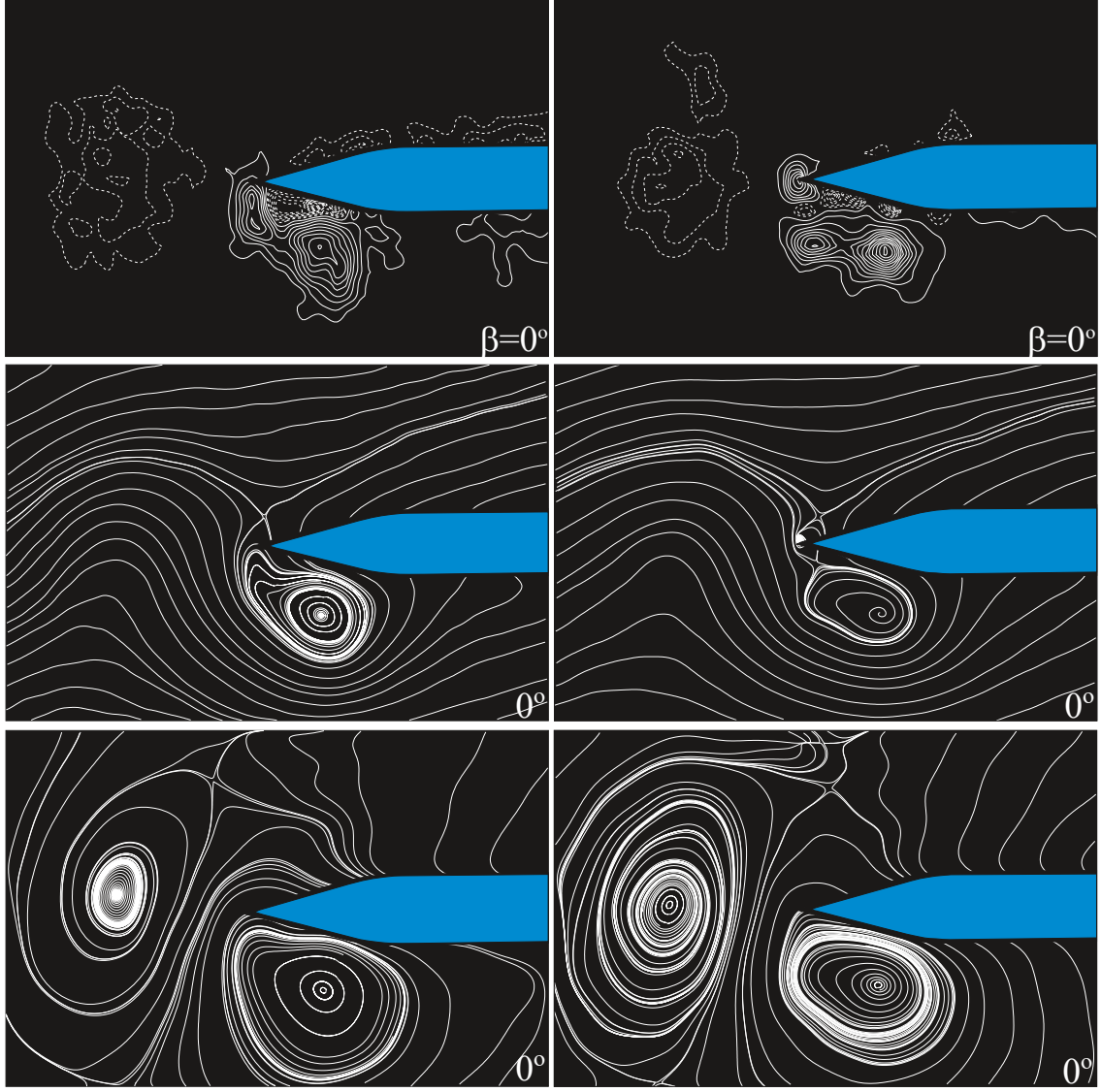
Figure 5.22: Reynolds number comparison of an oscillating leading-edge at \phi = 0^\circ with respect to an incident clockwise vortex. The left column shows Re = 6,250 , with |\omega_{\min}| = 5 \text{ sec}^{-1} , negative contour \Delta\omega = 5 \text{ sec}^{-1} , and positive contour \Delta\omega = 10 \text{ sec}^{-1} . The right column shows Re = 25,000 with |\omega_{\min}| = 20 \text{ sec}^{-1} , negative contour \Delta\omega = 20 \text{ sec}^{-1} , and positive contour \Delta\omega = 40 \text{ sec}^{-1} .
