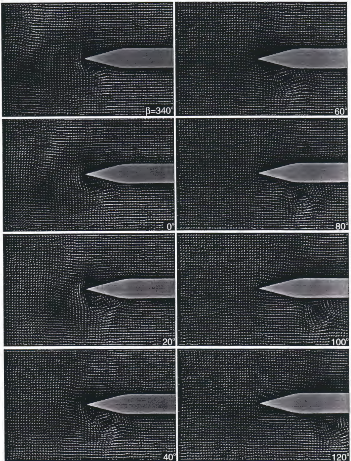
Figure 4.7: Instantaneous velocity field for a clockwise vortex impinging upon a stationary leading-edge at \alpha=0^\circ .
