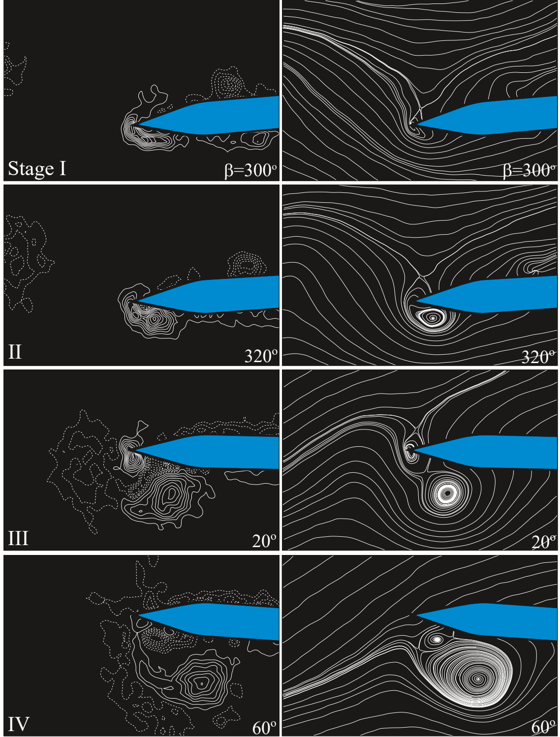
Figure 6.15: Instantaneous vorticity distributions and streamline patterns in the laboratory reference frame depicting the stages of tip vortex development for a leading-edge oscillating at \phi = 0^\circ with respect to an incident clockwise vortex. |\omega_{\min}| = 5 \text{ sec}^{-1} ; negative contour interval is \Delta\omega = 5 \text{ sec}^{-1} and positive contour interval is \Delta\omega = 10 \text{ sec}^{-1} . \text{Re} = 6,250 .
