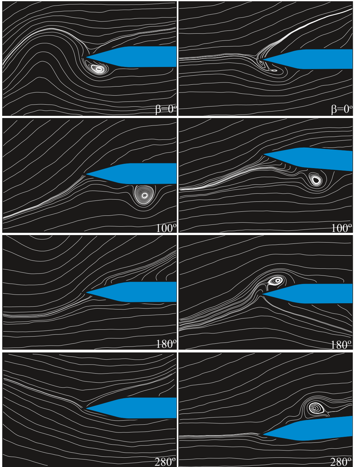
Figure 6.1: Comparison of streamline patterns in the laboratory reference frame for an incident vortex impinging a stationary leading-edge (left column) with those of a leading-edge oscillating without an incident vortex (right column). Re=6,250 .
