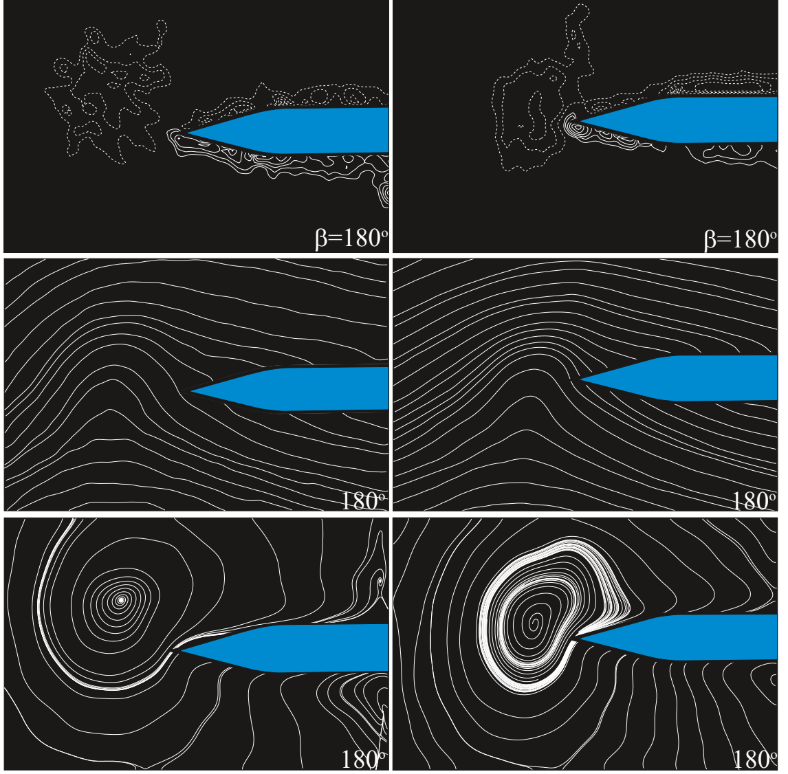
Figure 5.23: Reynolds number comparison of an oscillating leading-edge at \phi = 180^\circ with respect to an incident clockwise vortex. The left column shows Re = 6,250 with |\omega_{\min}| = 5 \text{ sec}^{-1} and contour interval \Delta\omega = 5 \text{ sec}^{-1} . The right column shows Re = 25,000 with |\omega_{\min}| = 20 \text{ sec}^{-1} and contour interval \Delta\omega = 20 \text{ sec}^{-1} .
