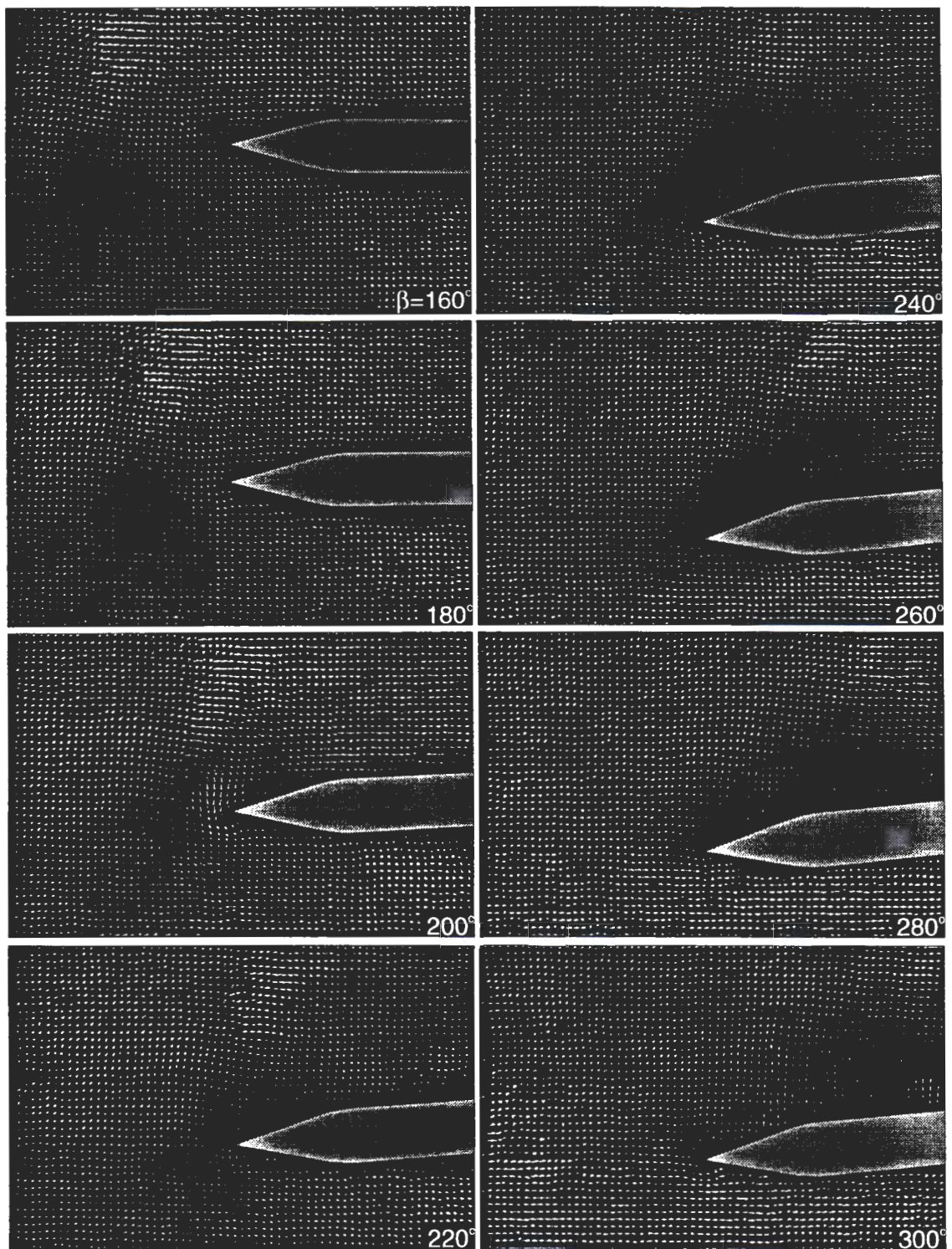
Figure 5.20: Instantaneous velocity field of an oscillating leading-edge at \phi = 180^\circ with respect to an incident clockwise vortex. Re = 6,250 .
