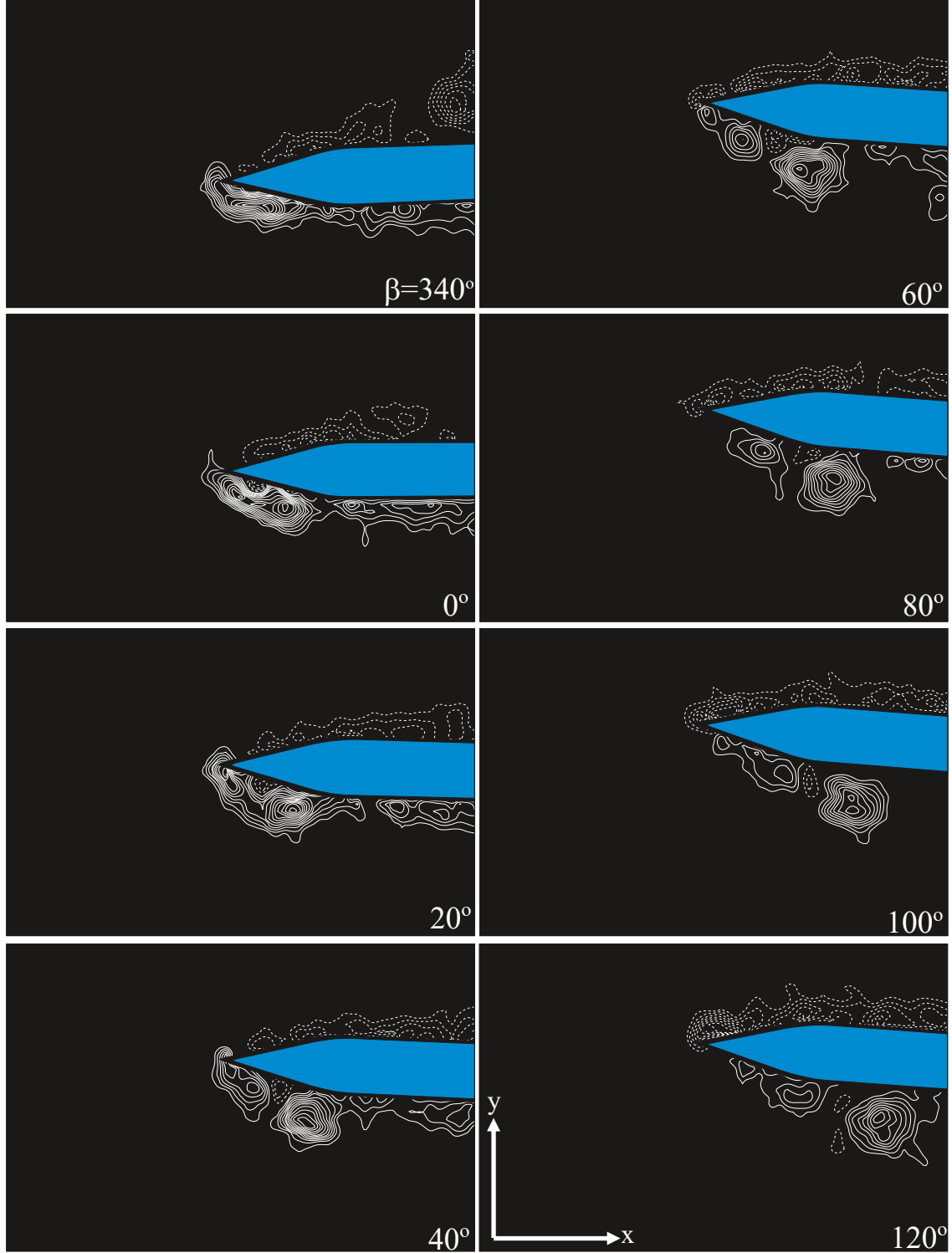
Figure 5.1: Instantaneous vorticity distributions for an oscillating leading-edge without an incident vortex. |\omega_{\min}| = 5 \text{ sec}^{-1} \Delta\omega = 5 \text{ sec}^{-1} . \text{Re} = 6,250 .
