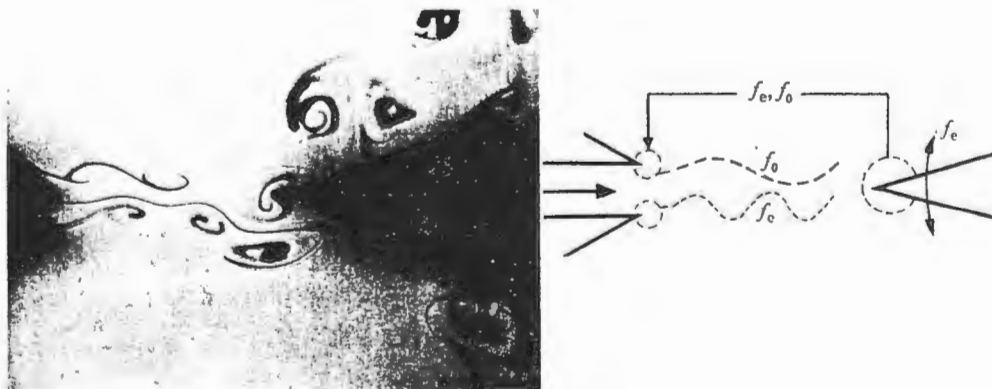
b) Jet impinging upon the oscillating edge ( f_e = 4f_0 ).
