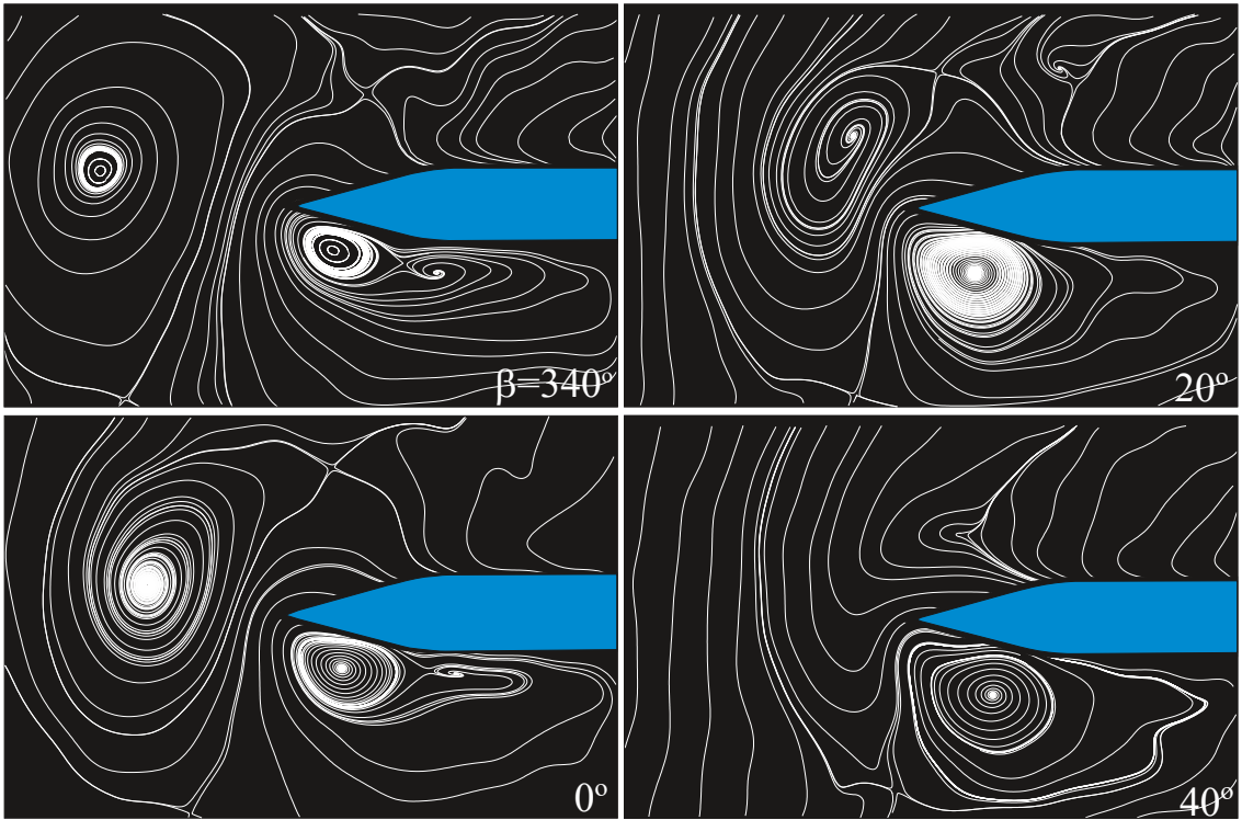
Figure 4.5: Streamline patterns in a reference frame moving at U/U_\infty = 0.9 for a clockwise vortex incident upon a stationary leading-edge.
