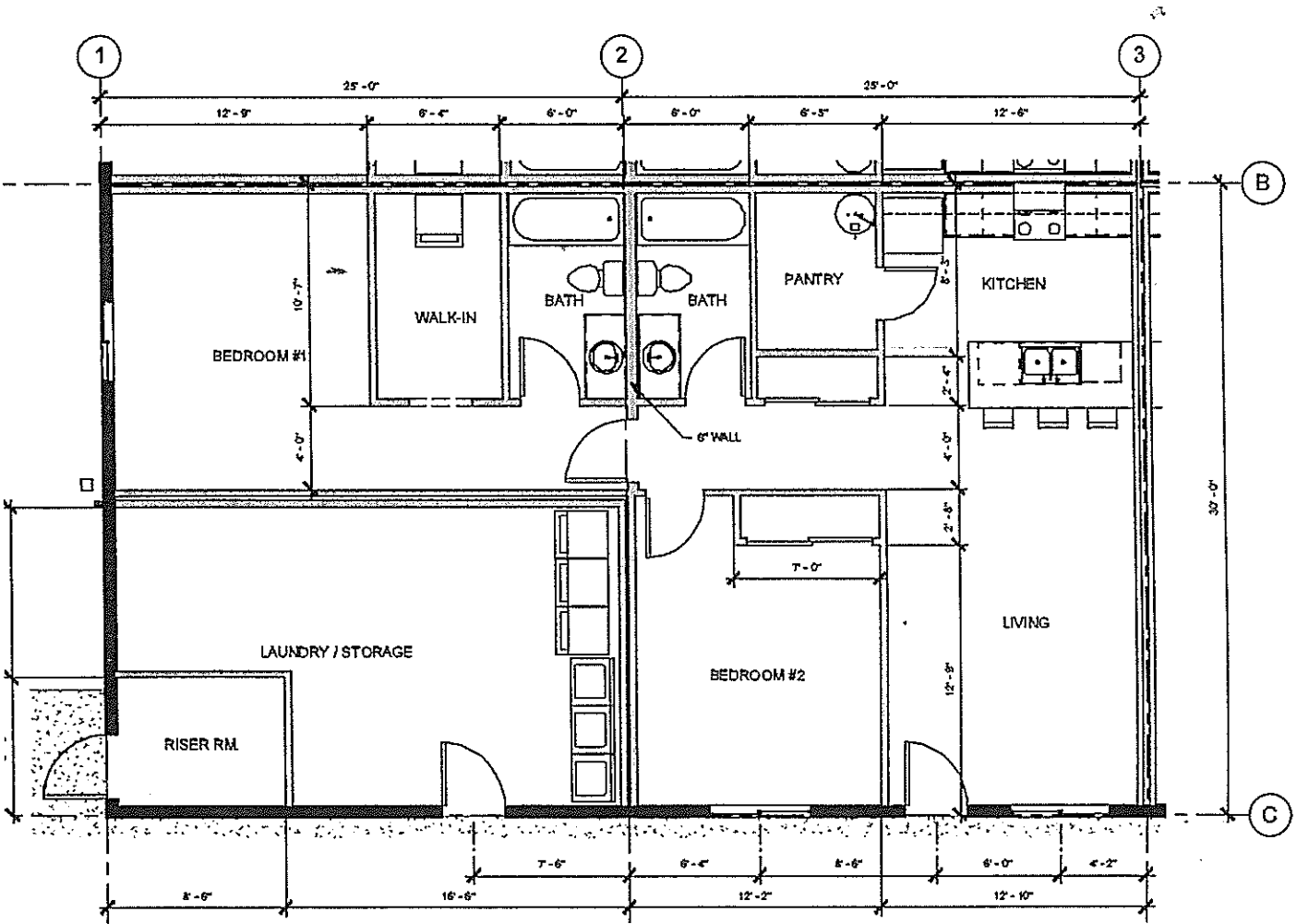
2 ENLARGED 2 BEDROOM UNIT 1/4" = 1'-0"
