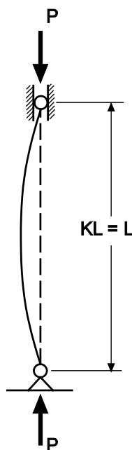
Figure C-E2-4 Overall Column Buckling
