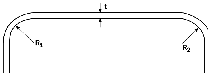
Figure C-B4.1-1 Corner Radius
