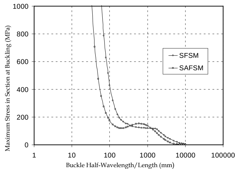
Figure C-2.2.5-2 Examples of Shear Elastic Buckling Analysis by Spline Finite Strip Method (SFSM) Similar to Shell Finite Element Solution, and a Generalized Version of the Semi-Analytical Finite Strip Method (SAFSM)
