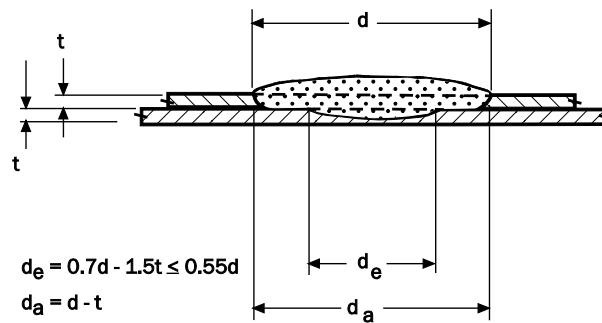
Figure J2.3.2.2-1 Arc Seam Weld – Sheet to Sheet
