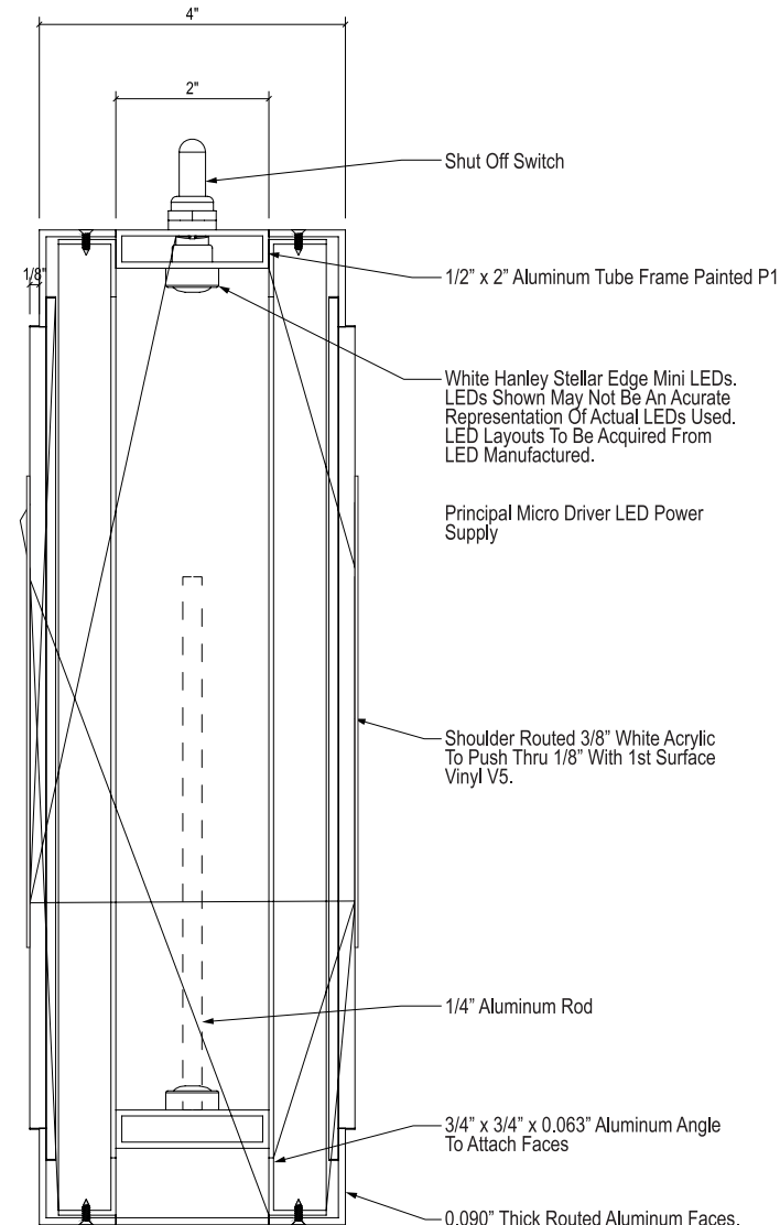
SECTION A
