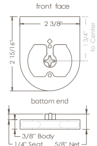
FLOATING/OUTSIDE MOUNT: DRIVE SIDE SHA-B4XX
