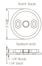
INSIDE/JAMB MOUNT: IDLER SIDE SHA-B1XX
