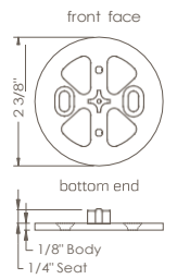
INSIDE/JAMB MOUNT: DRIVE SIDE SHA-B2XX
