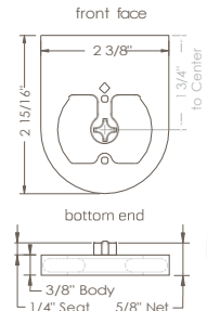
FLOATING/OUTSIDE MOUNT MANUAL: DRIVE SIDE SHA-B4MANUALXX
