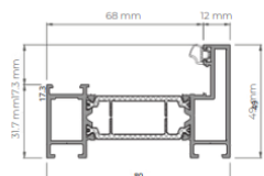
Sash With Gasket
