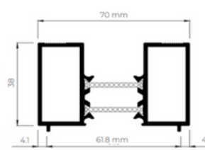
HEAD EXTENSION 38 MM
