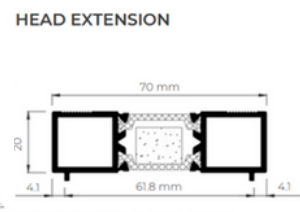
HEAD EXTENSION 20 MM
