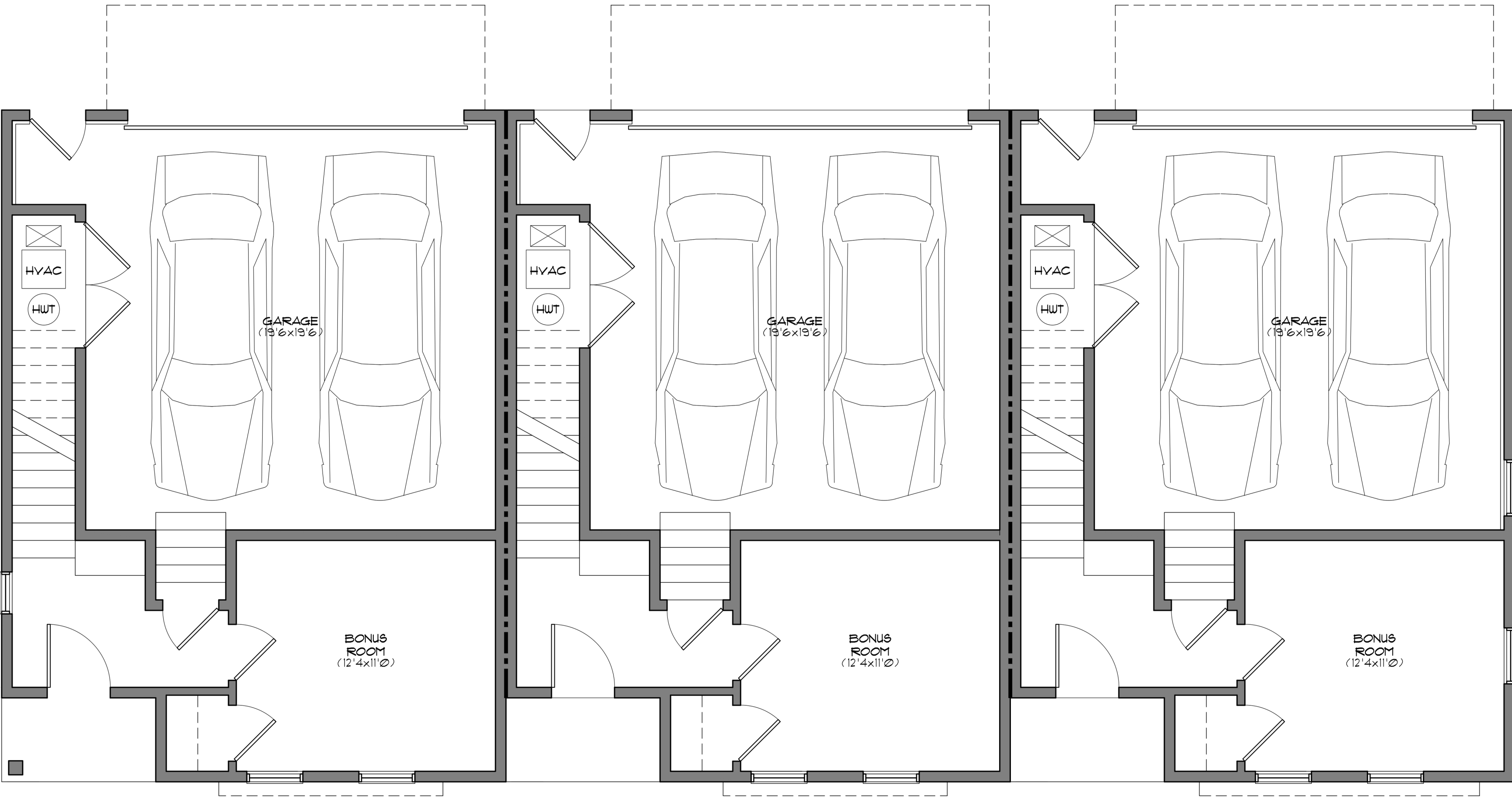
UNIT 6 FIRST FLOOR
