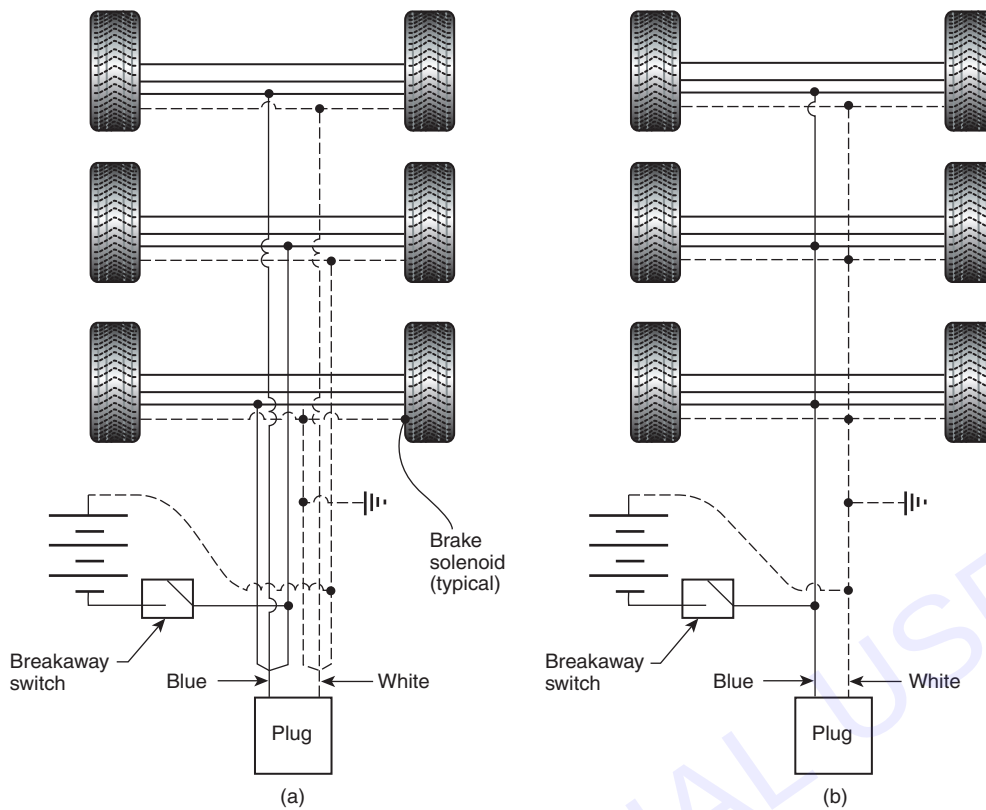
FIGURE 8.4.1.7 Brake Wiring Diagram. [© 2014 Canadian Standards Association]
