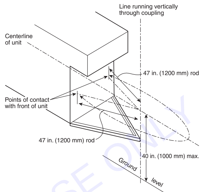
Δ FIGURE A.8.1.2.2 Method of Determining Shortest Tongue or A-Frame. [© 2014 Canadian Standards Association]
