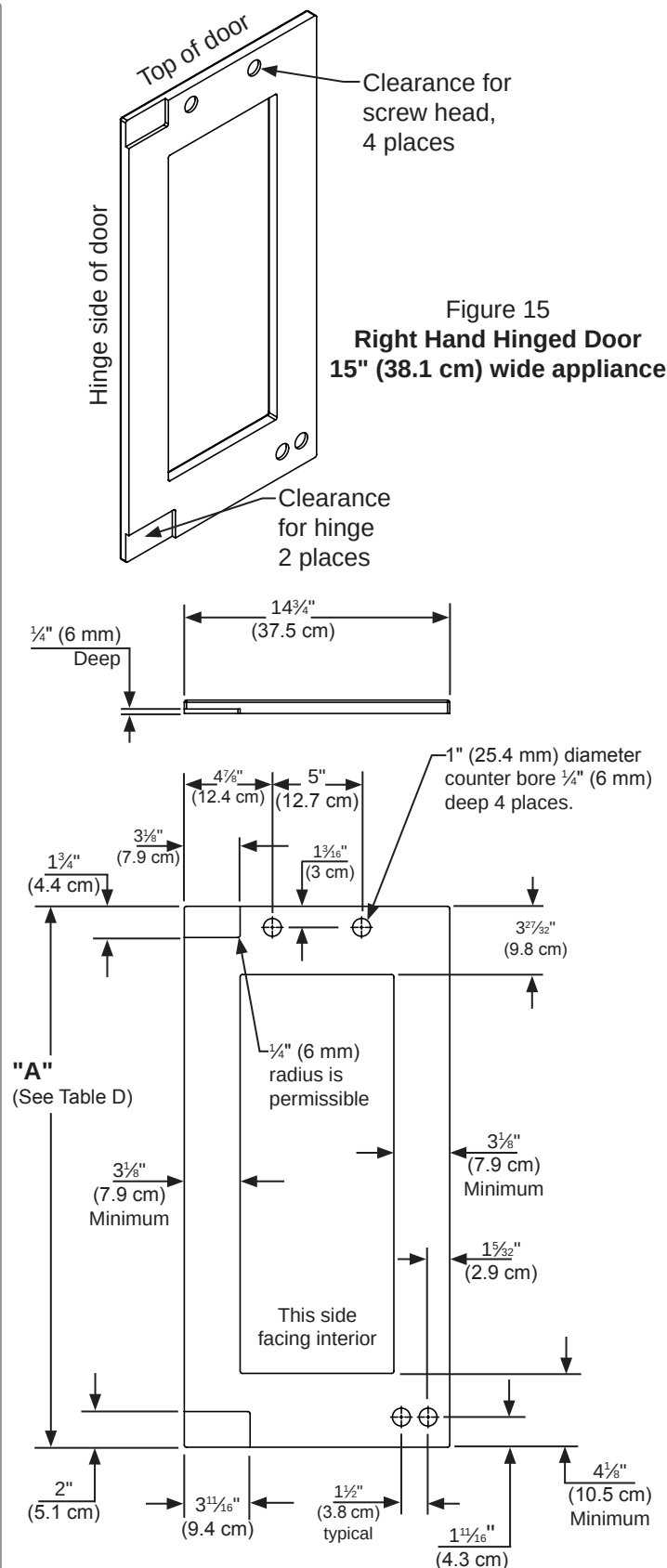
Figure 16 Right Hand Hinged Door 15" (38.1 cm) wide appliance
