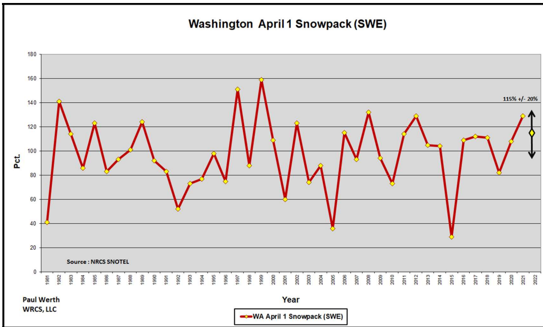
Figure 1. Washington April 1 SWE 1981-2021 and predicted 2022.
