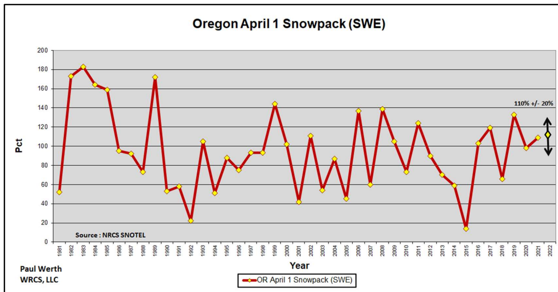
Figure 2. Oregon April 1 SWE 1981-2021 and predicted 2022.
