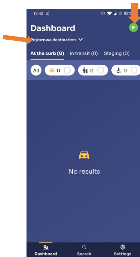
Image 1 Automatic Request
