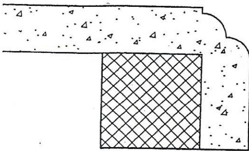
R-250 1/4" STEPPED B.B. W/ FILLET
