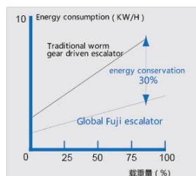
Schematic diagram of the efficiency of helical gear reducer compared to worm gear reducer
