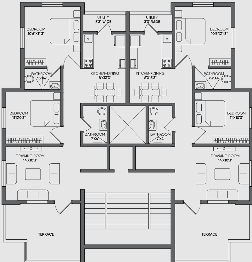
Typical Floor Plan for Third Floor
