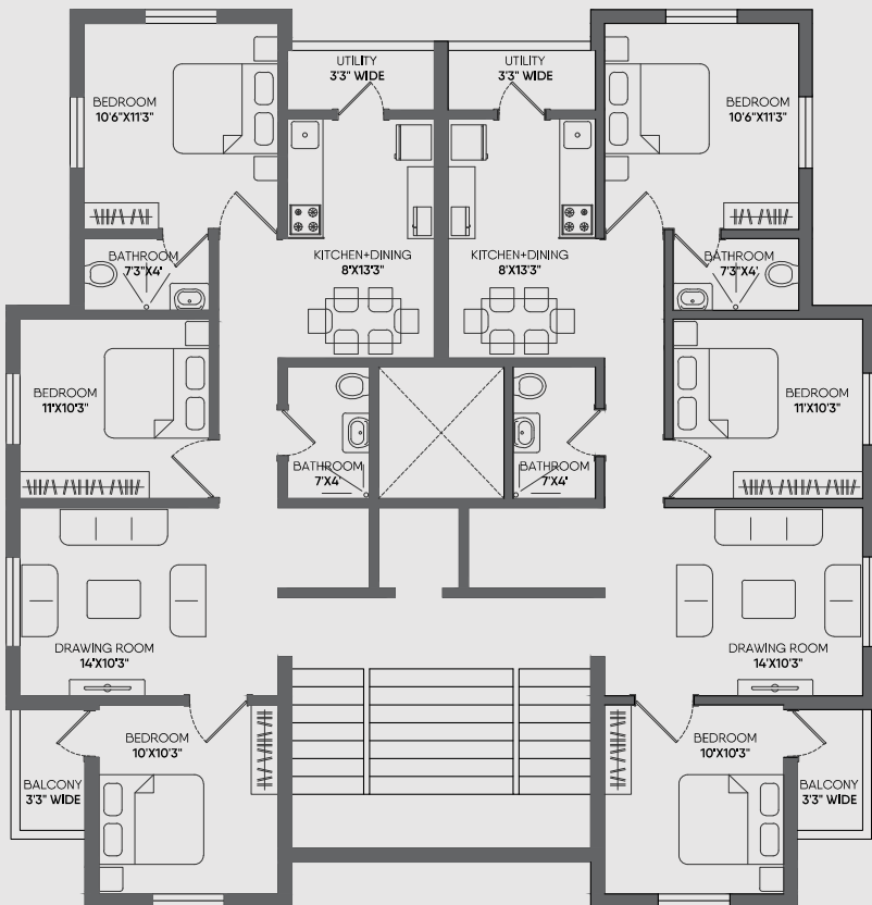
Typical Floor Plan for First & Second Floors
