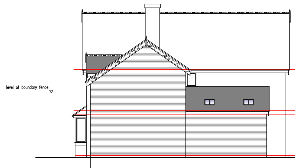
Proposed Side (NE) Elevation
