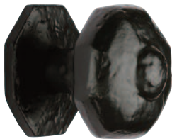
TC350 Centre Door Knob Base diameter: 64mm Knob diameter: 63mm Projection: 64mm
