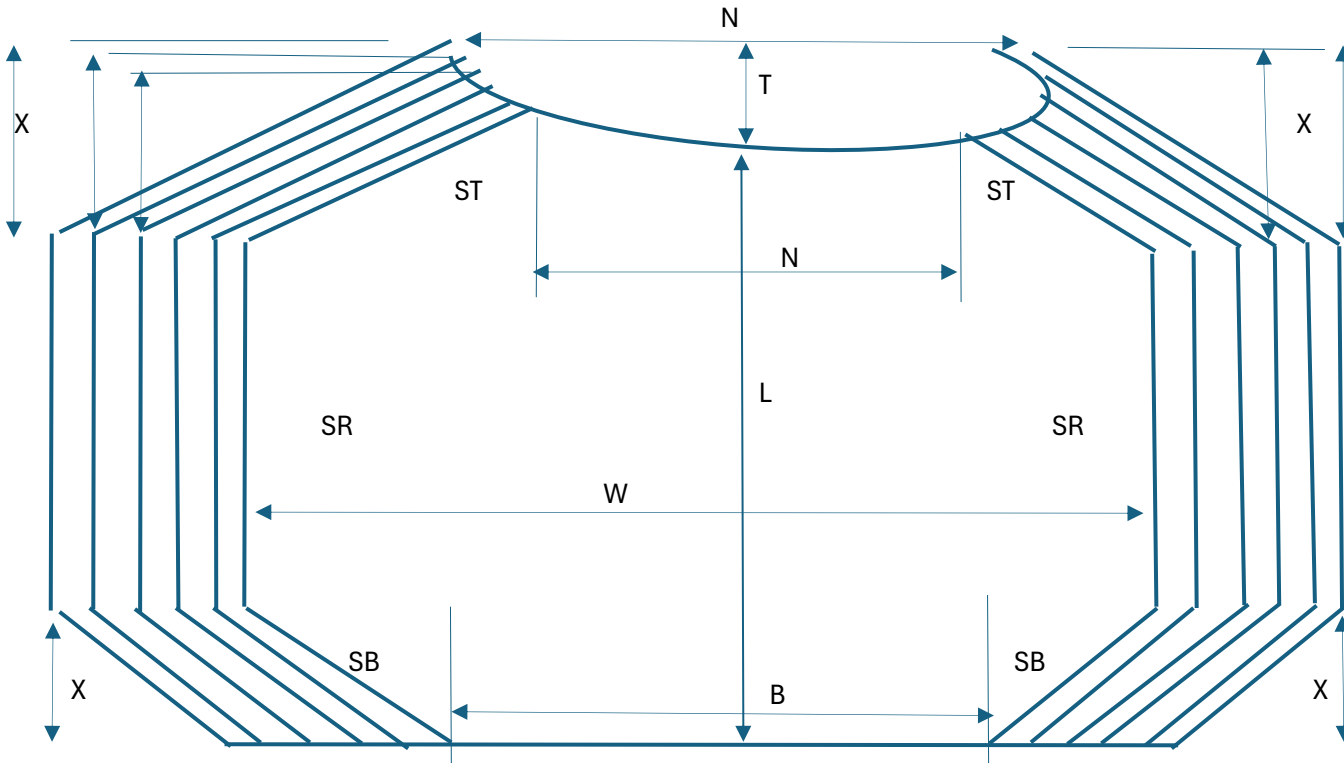
CHART "C" FOR MAKING PATTERNS TO CUT MULTIPLE DTS SKIRTS FOR ANY SELECTED TREE SIZE
