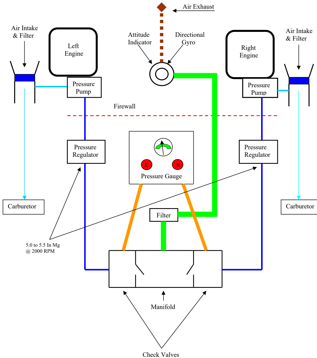
BE-76 PRESSURE SYSTEM SCHEMATIC
