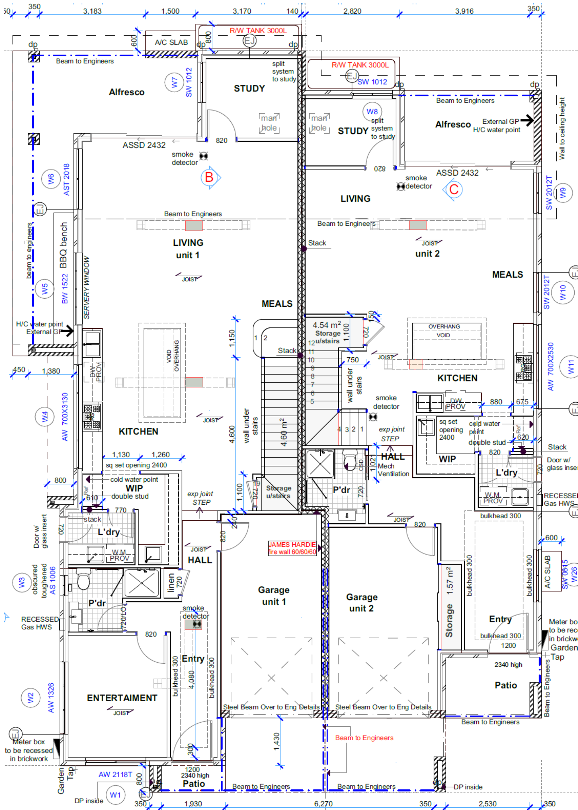
GROUND FLOOR
