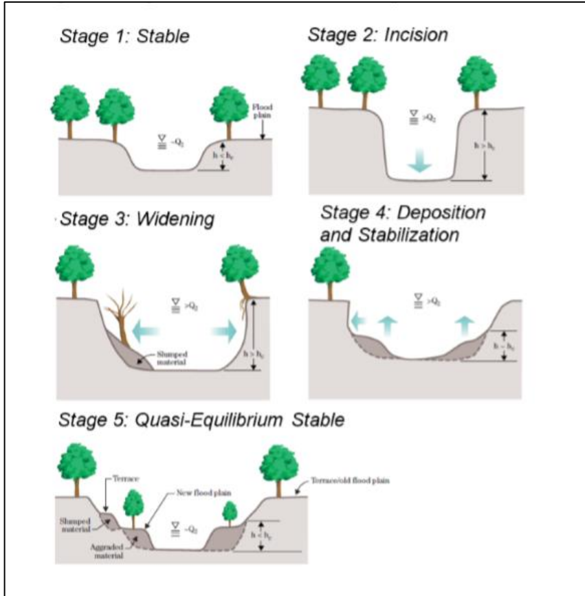
Channel evolution (modified NRCS, 2007)
