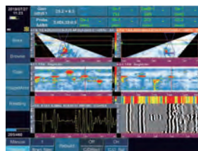
Simultaneous Display of PAUT & TOFD
