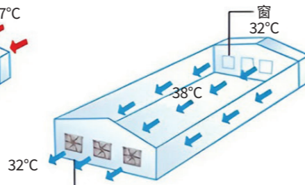
负压抽风机 Negative pressure fan system
