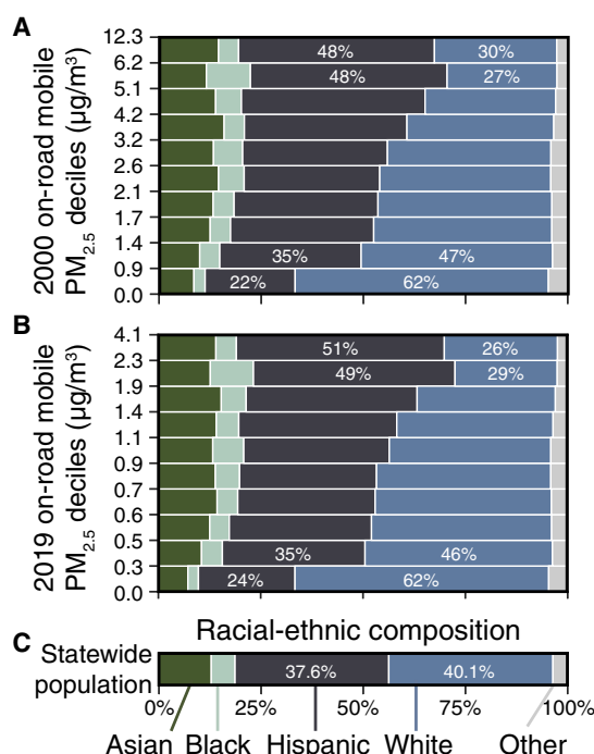
Fig. 2. Racial-ethnic population distribution by exposure decile. Differences in the racial-ethnic composition of the California population exposed to each decile of the distribution of PM 2.5 attributable to on-road mobile sources in (A) 2000 and (B) 2019. The statewide population is binned into 10 groups of equal population of PM 2.5 exposure attributable to the full vehicle fleet. At all years in our assessment, Hispanic Californians are strongly overrepresented among the highest PM 2.5 exposure deciles (and underrepresented in the lowest exposure deciles). The opposite pattern holds for white Californians. Data are plotted for individual vehicle types and the analysis midpoint year (2010) in the Supplementary Materials.
