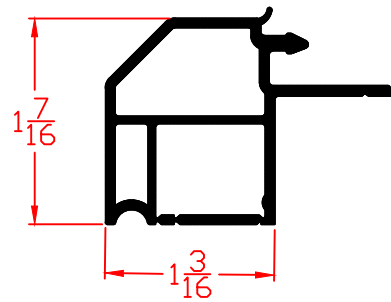
5917 Brick Mould w/ J-Channel
