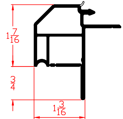
5907 Brick Mould w/Windbreak & J-Channel
