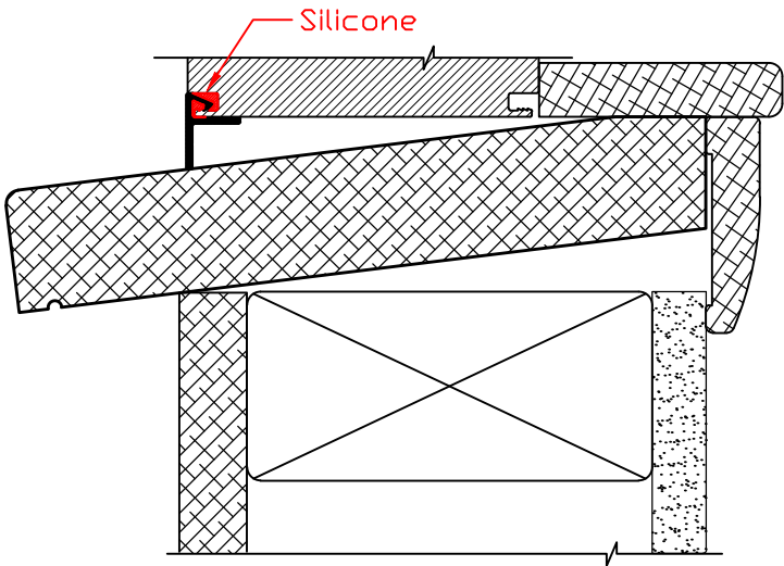
Sill Extender shown configured for slope sill.
