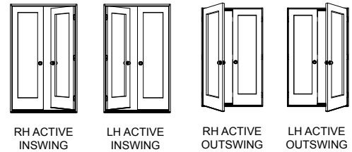
OSLI VIEWED FROM EXTERIOR, HANDING BY KNOB F = FIXED L = LEFT HAND R = RIGHT HAND
