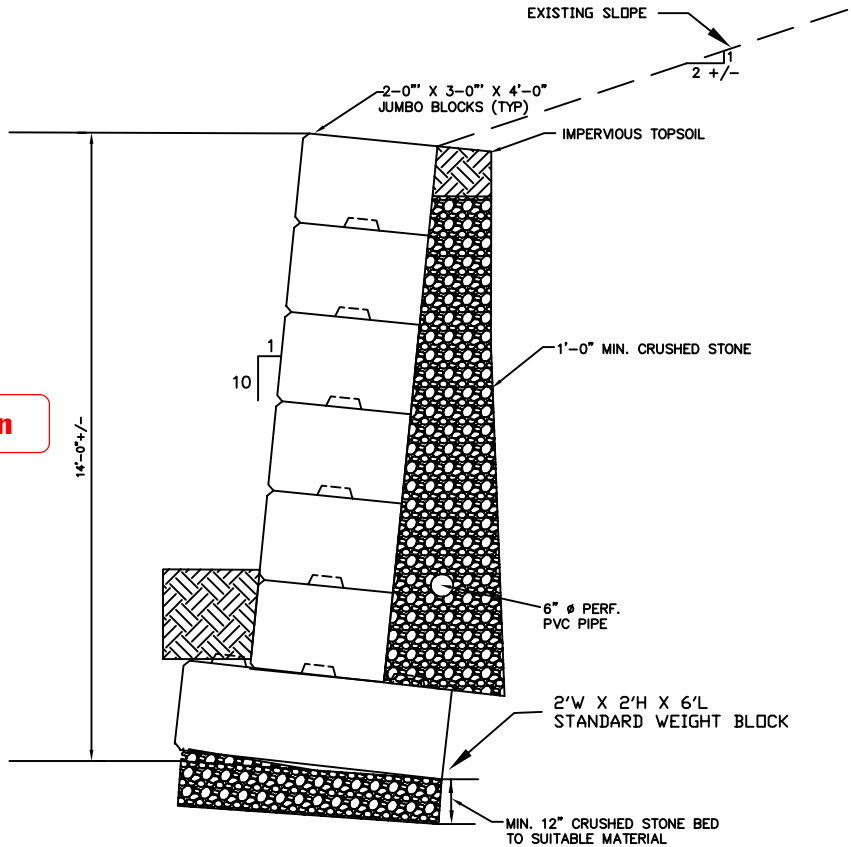
GRAVITY WALL #2 DESIGN SECTION – DESIGN HEIGHT 14'-0"
