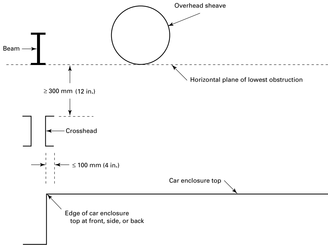
Fig. G-6 Additional Top-of-Car Clearance [2.4.7.1(b)]
