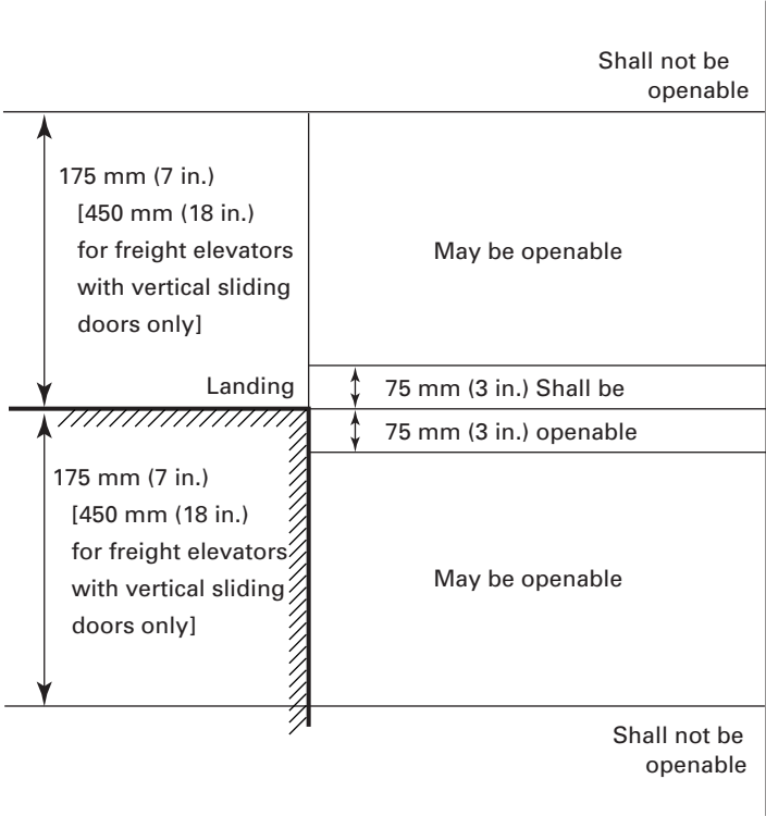
Fig. B-1 Unlocking Zone (2.12.1 and 2.14.5.7)
