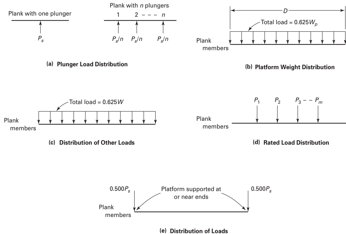
Fig. 8.2.9.1.3 Load Distribution
