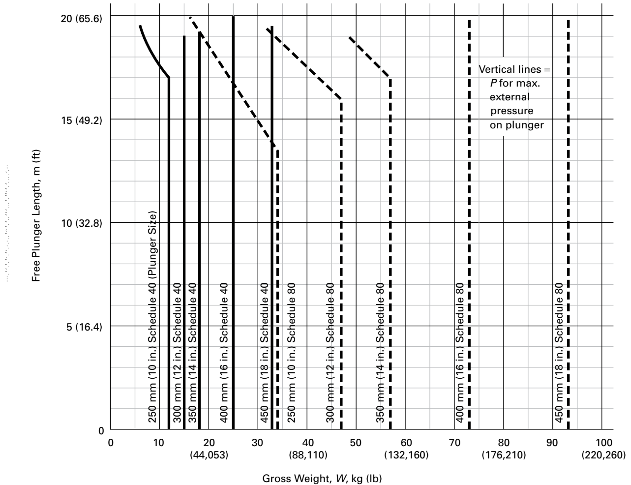
Fig. 8.2.8.1.1 Allowable Gross Loads (Cont'd)
