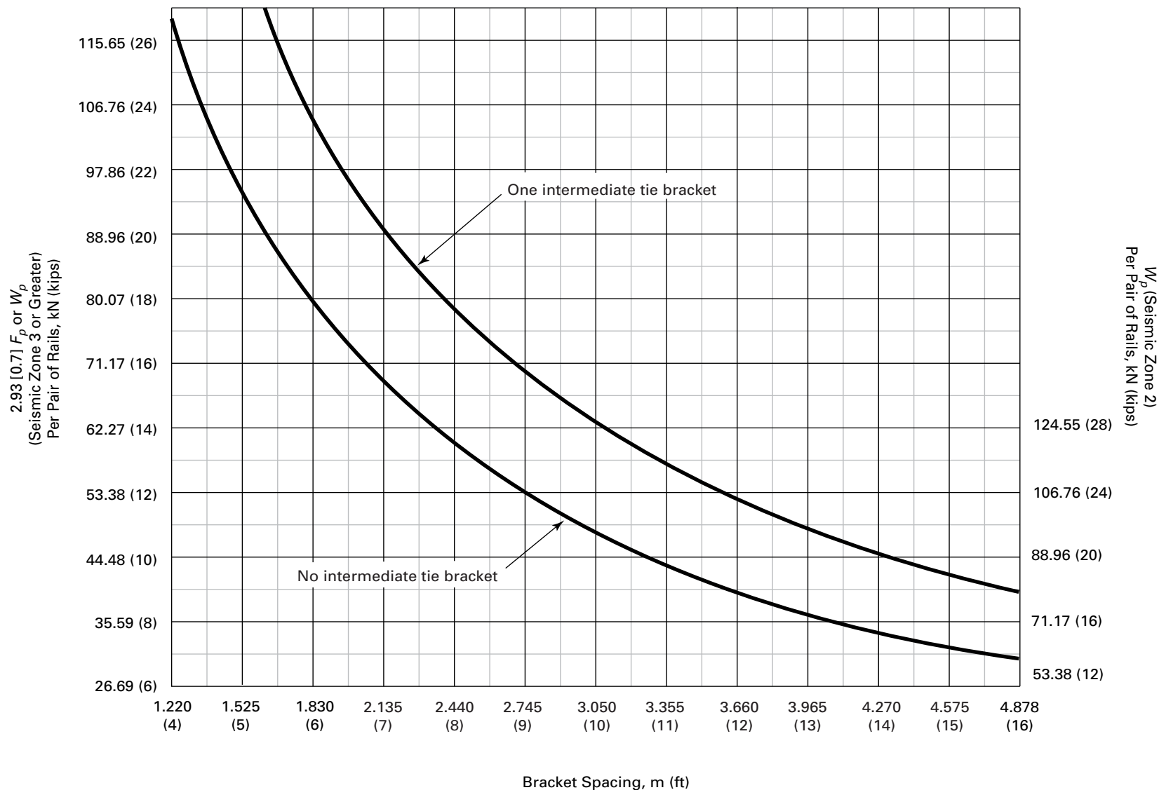
Fig. 8.4.8.2-2 16.5 kg/m (11 lb/ft) Guide-Rail Bracket Spacing
