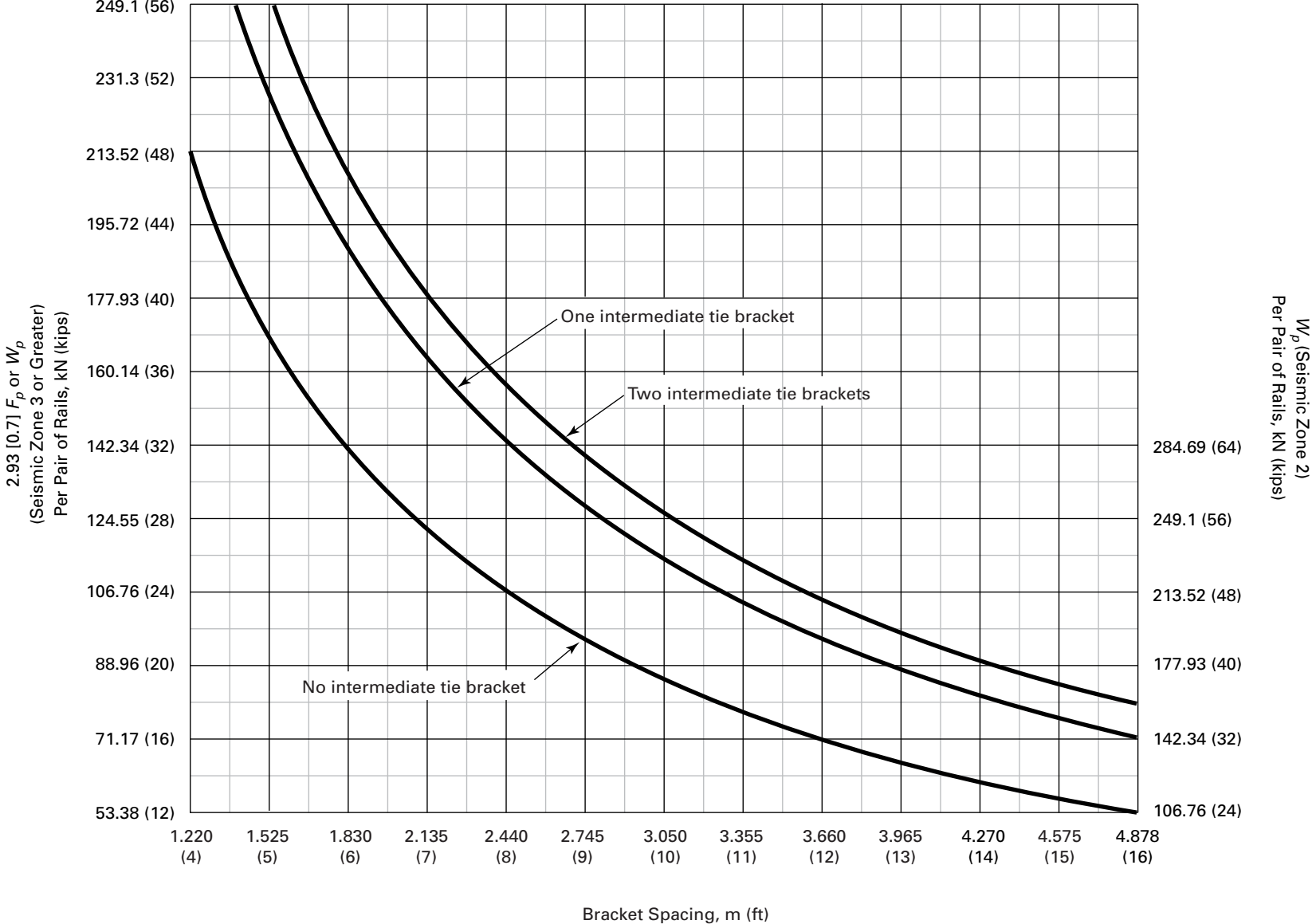
Fig. 8.4.8.2-5 27.5 kg/m (18.5 lb/ft) Guide-Rail Bracket Spacing
