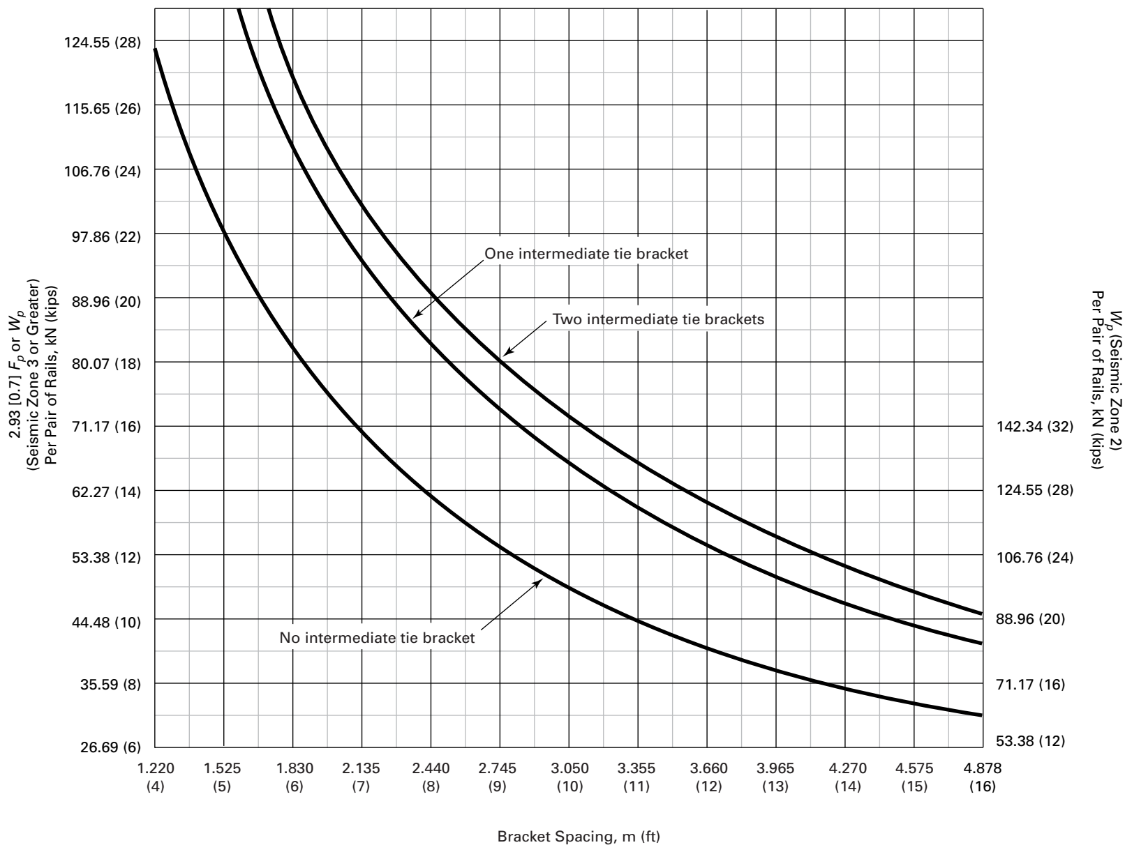
Fig. 8.4.8.2-3 18 kg/m (12 lb/ft) Guide-Rail Bracket Spacing
