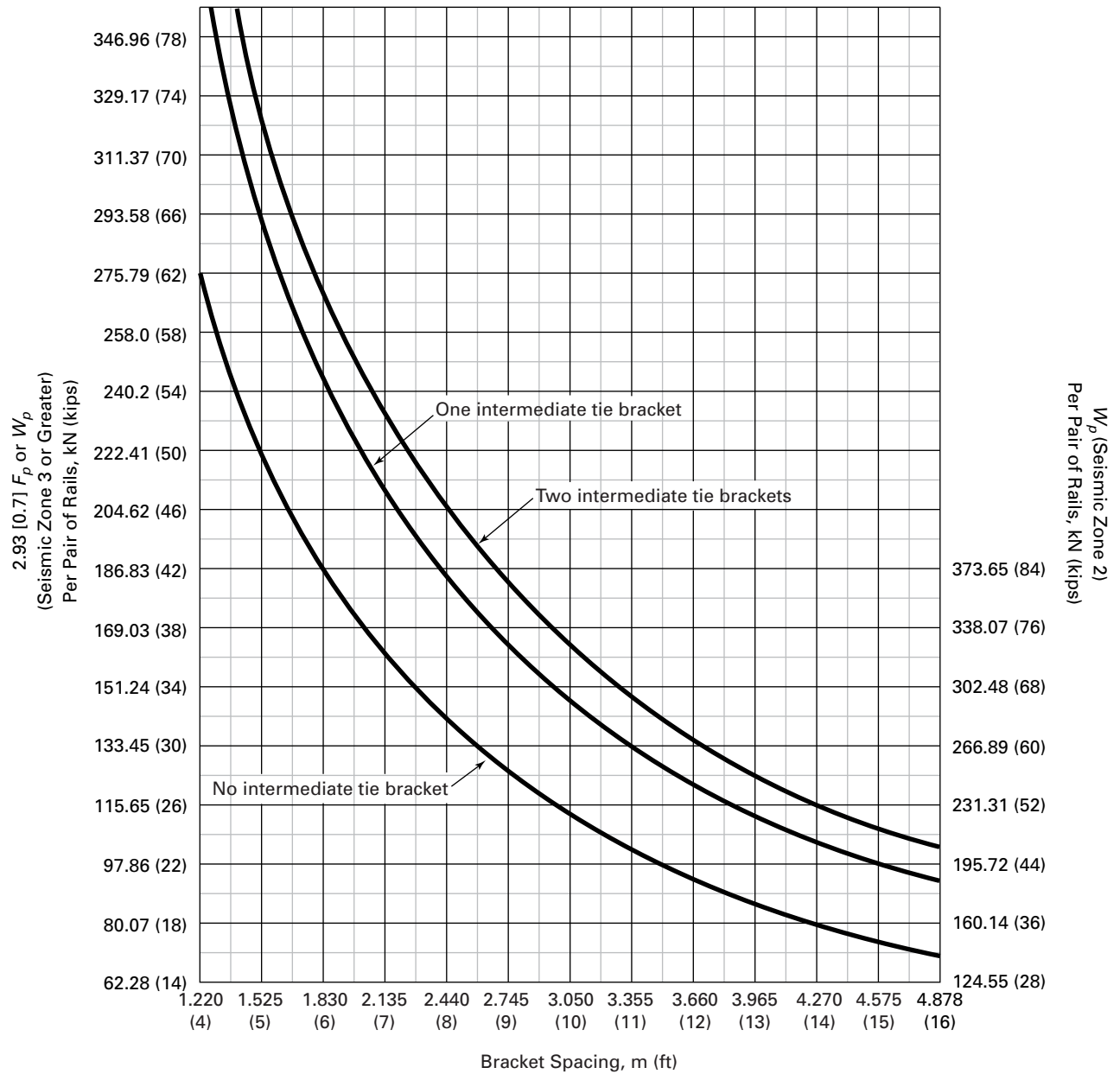
Fig. 8.4.8.2-6 33.5 kg/m (22.5 lb/ft) Guide-Rail Bracket Spacing
