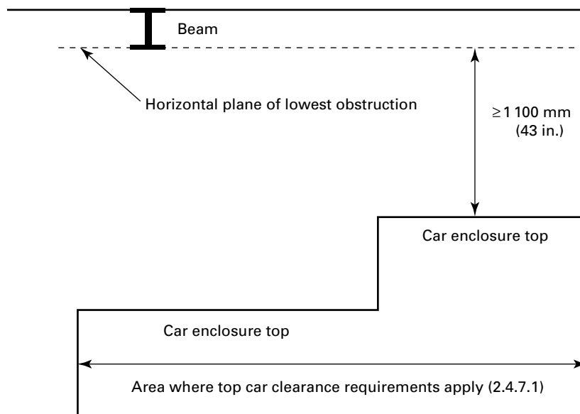
Fig. G-2 Additional Top-of-Car Clearance Requirements (2.4.7.1)
