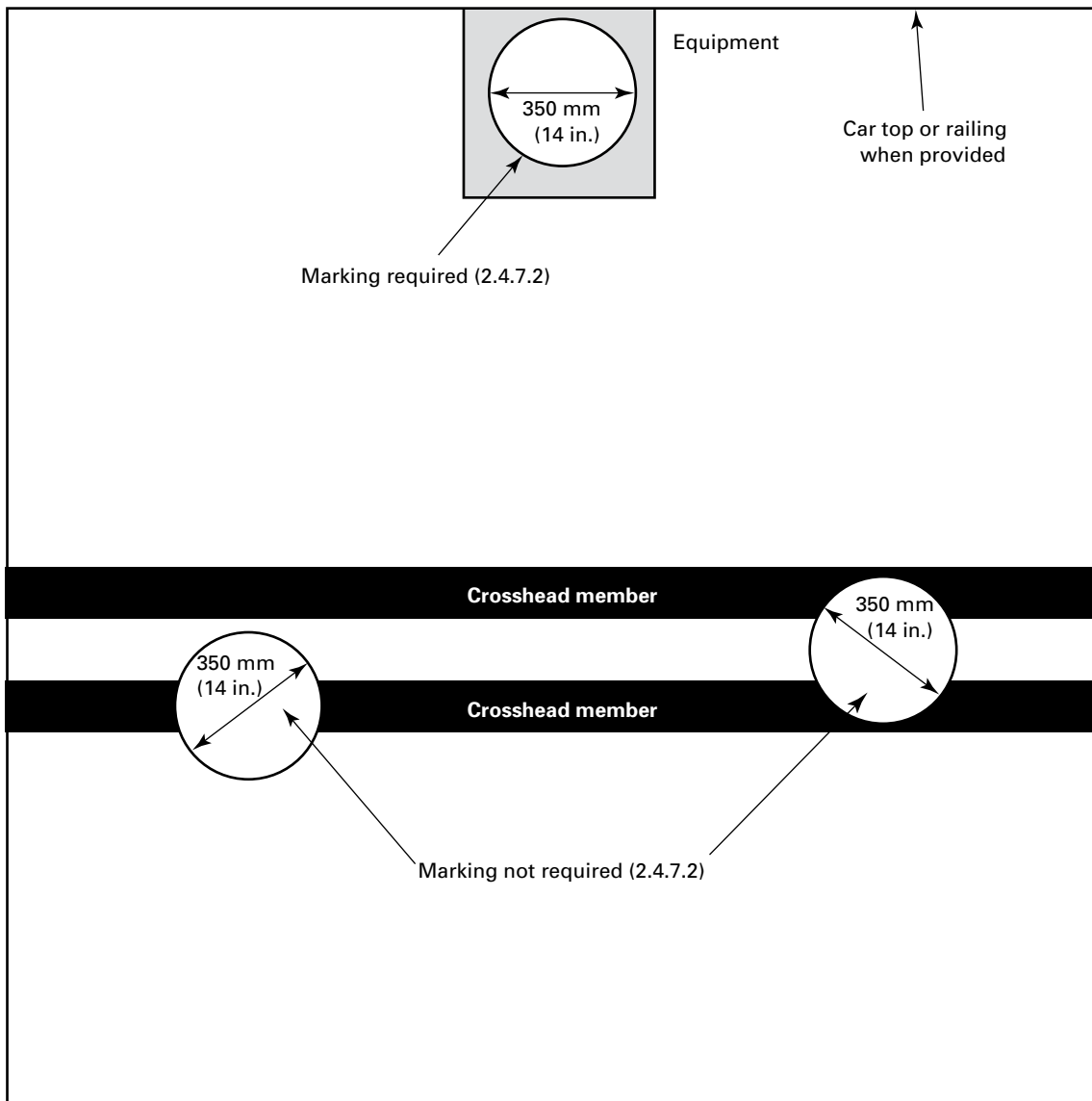
Fig. G-4 Additional Top-of-Car Marking Requirements (2.4.7.2)
