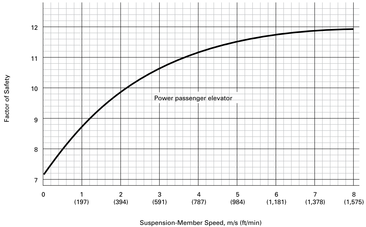
Fig. 8.2.7 Minimum Factors of Safety of Suspension Members of Power Passenger and Freight Elevators
