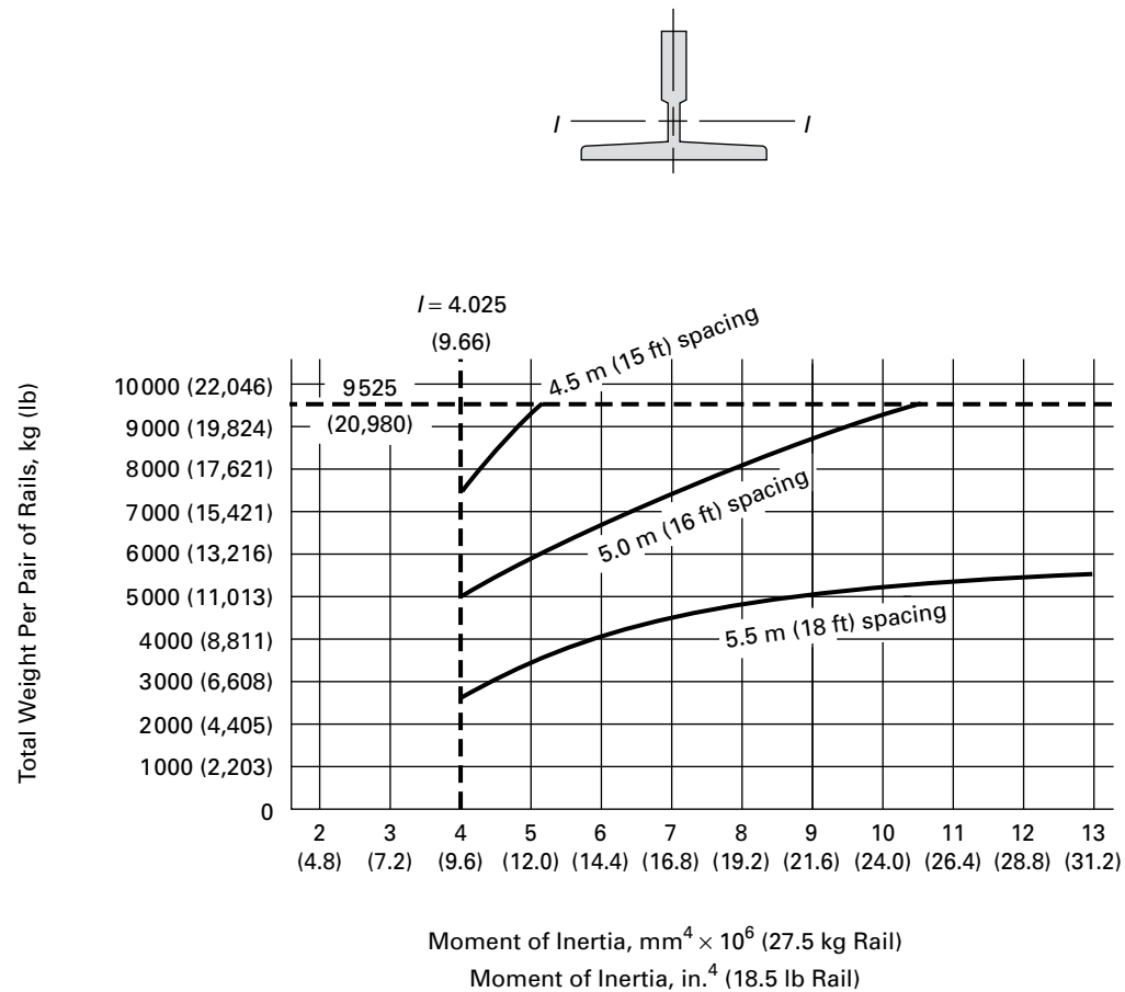
Fig. 2.23.4.1-2 Minimum Moment of Inertia About x-x Axis for a Single Guide Rail With Its Reinforcement (Cont'd)
