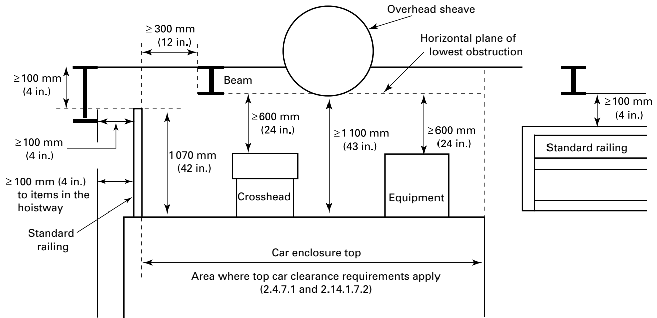
Fig. G-1 Top-of-Car Clearance Requirements (2.4.7.1 and 2.14.1.7.2)
