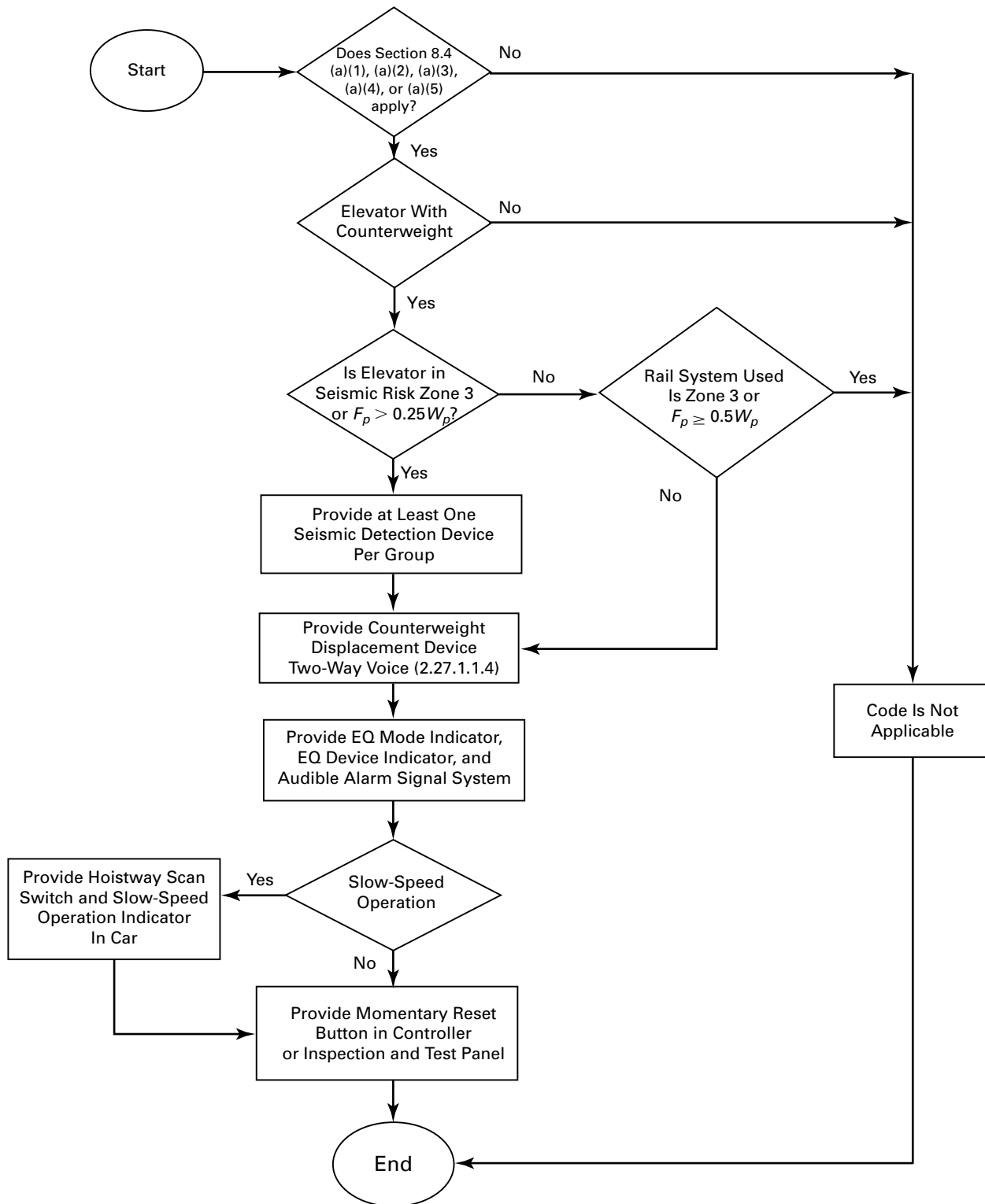
Fig. 8.4.10.1.1 Earthquake Elevator Equipment Requirements Diagrammatic Representation
