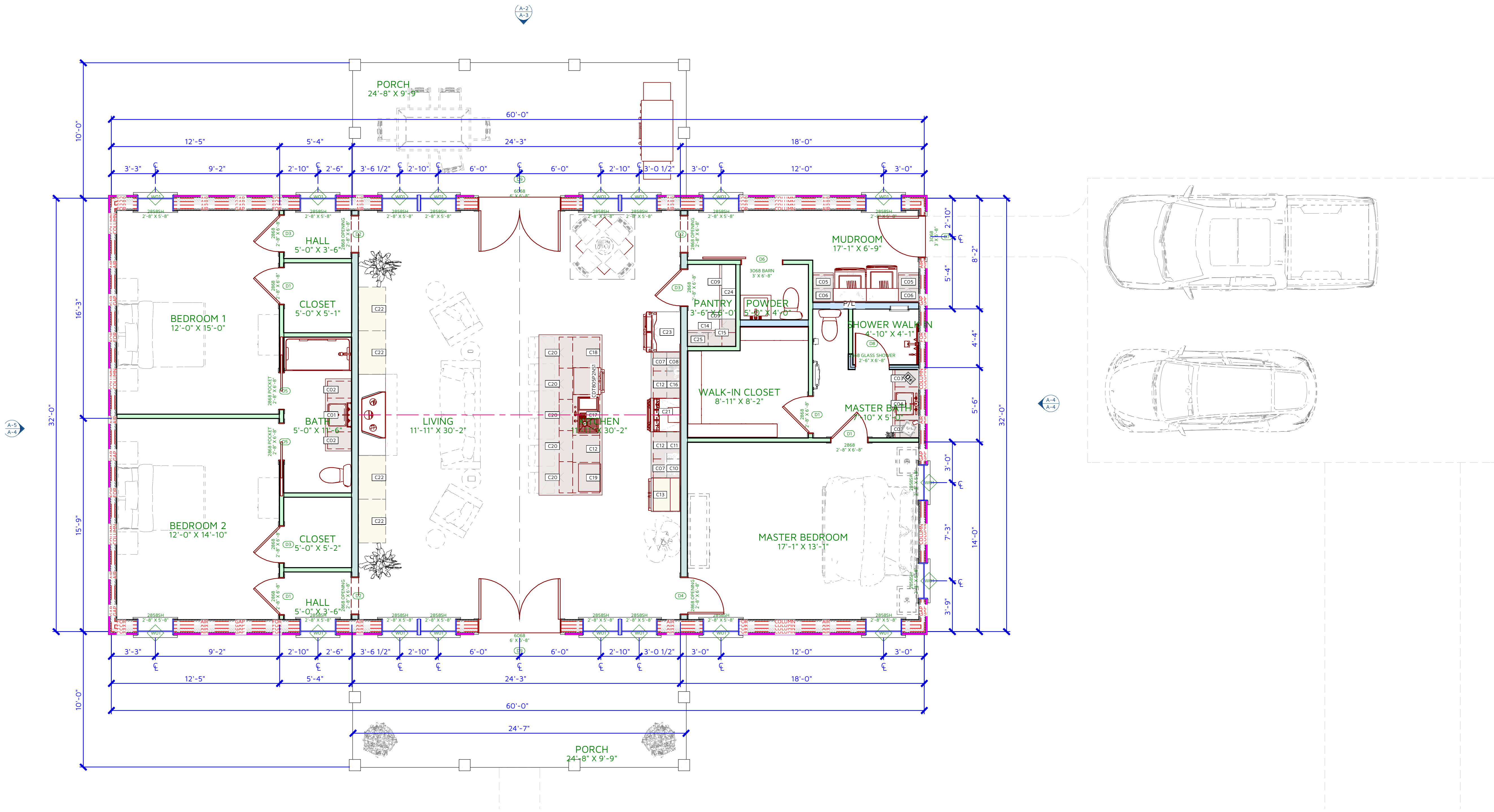
A-1.0 FLOOR PLAN FIRST FLOOR 1/4 IN = 1 FT
