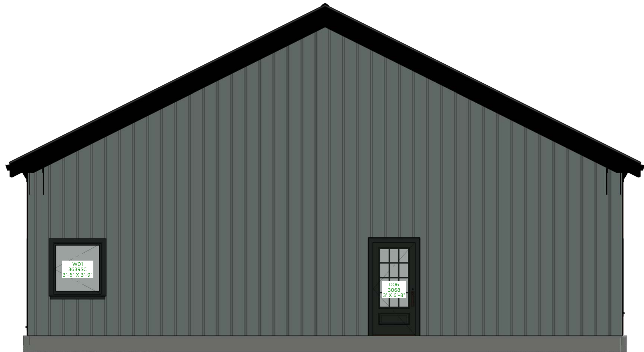
A-5 A-3 EXTERIOR ELEVATION LEFT 1/4 IN = 1 FT
