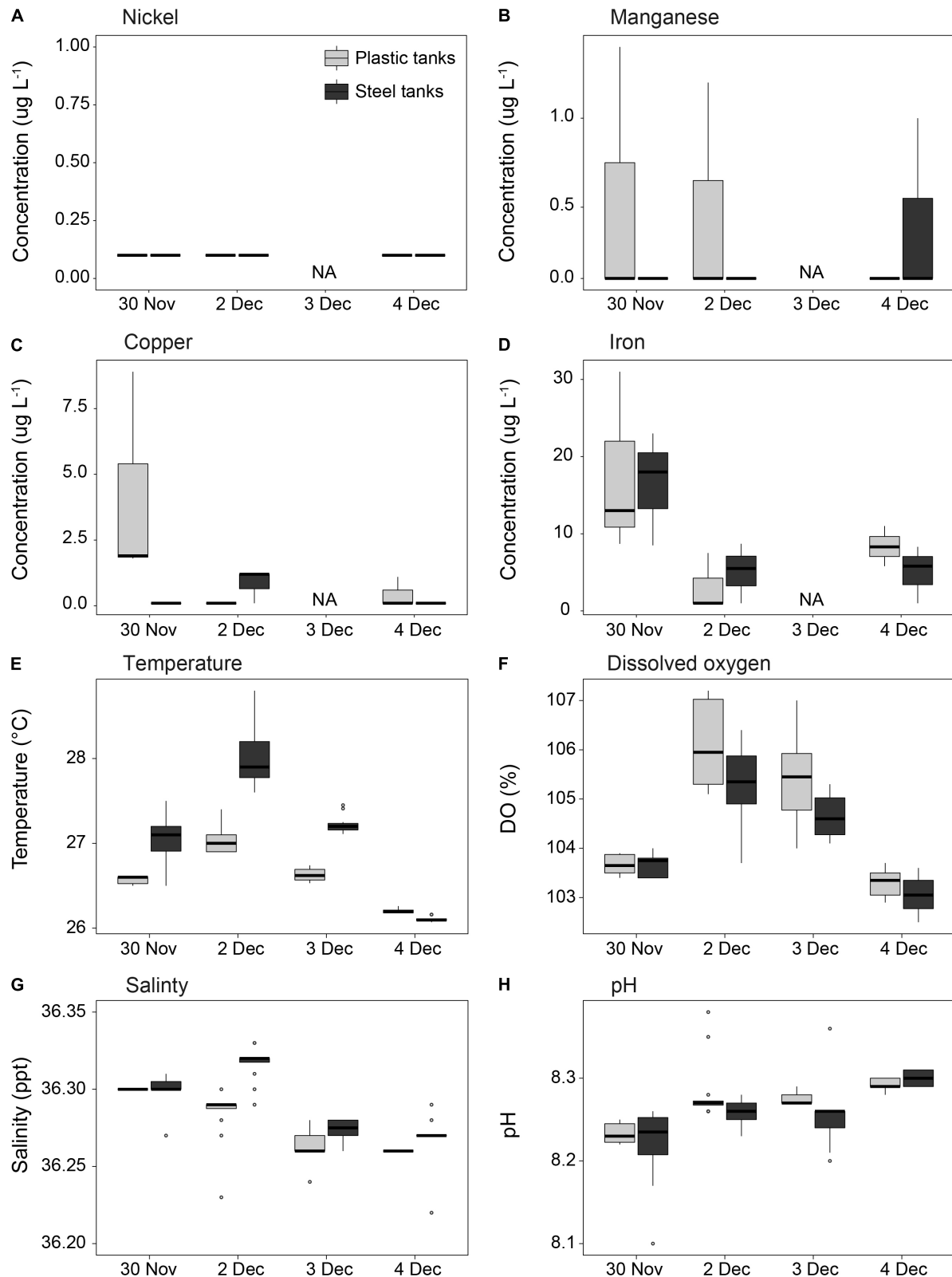
FIGURE 6 | Measurements of (A–D) dissolved metal concentrations and (E–H) water quality in the culture tanks throughout the duration of the coral larvae culturing period. The first batch of spawn slicks were pumped into the culture tanks at 00:30 am on Nov 30. Light gray = plastic tanks; dark gray = steel tanks ( n = 3 per tank type for A–D; n = 6 per tank type for E–H; NA = no samples for A–D).
