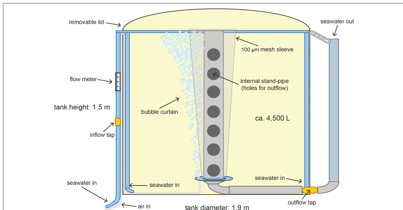
FIGURE 3 | Detail of tank design for flow-through rearing of the coral larvae. The water is circulated by the two opposing inflows and mixed from the flow of bubbles. The cone shaped mesh provides a large surface area that prevents larvae being lost to the outflow holes on the internal standpipe while the bubble curtain prevents them sticking to the mesh.
