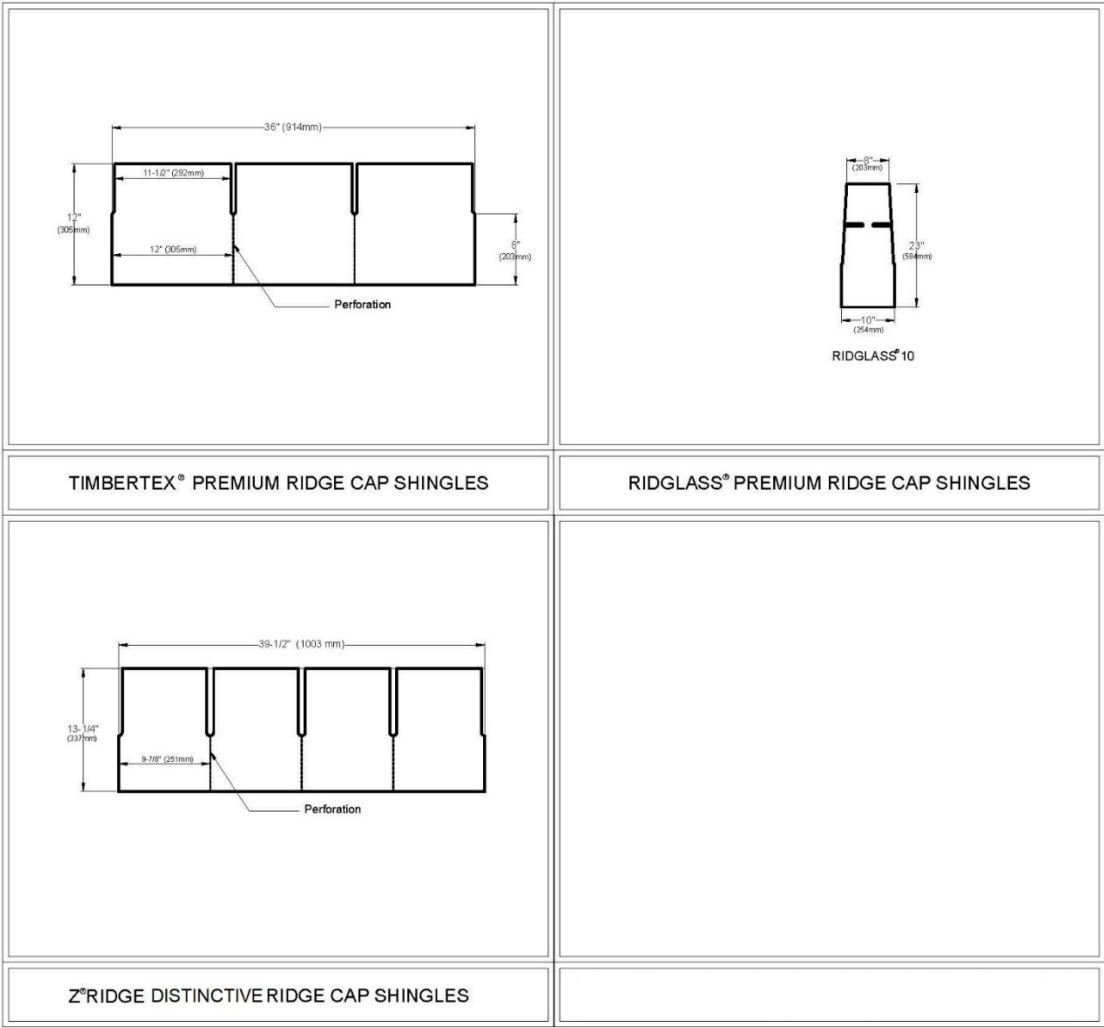
FIGURE 2—STARTER AND RIDGE SHINGLES (continued)
