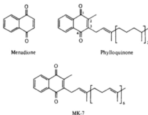
Figure 8 Chemical structures of three major forms of vitamin K.
