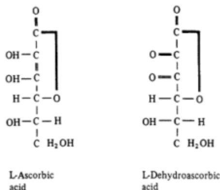
Figure 9 The reduced and oxidized forms of ascorbic acid.
