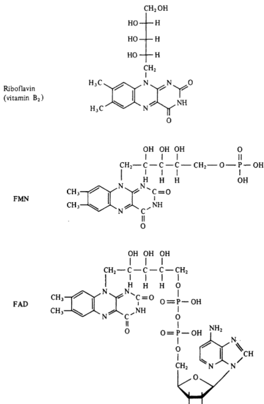
Figure 12 Chemical structures of riboflavin and its coenzyme forms.
