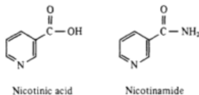
Figure 11 Chemical structures of major niacin-active compounds.
