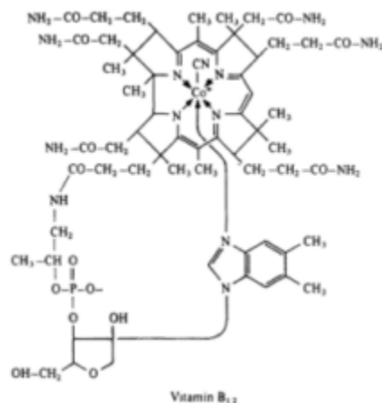
Figure 17 Chemical structure of the cyano form of vitamin B 12 (cyanocobalamin).
