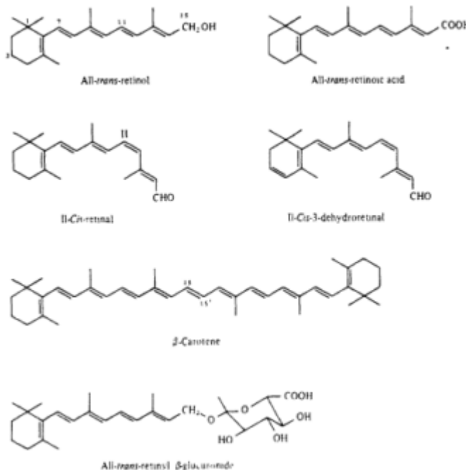
Figure 1 Major compounds of the vitamin A group.
