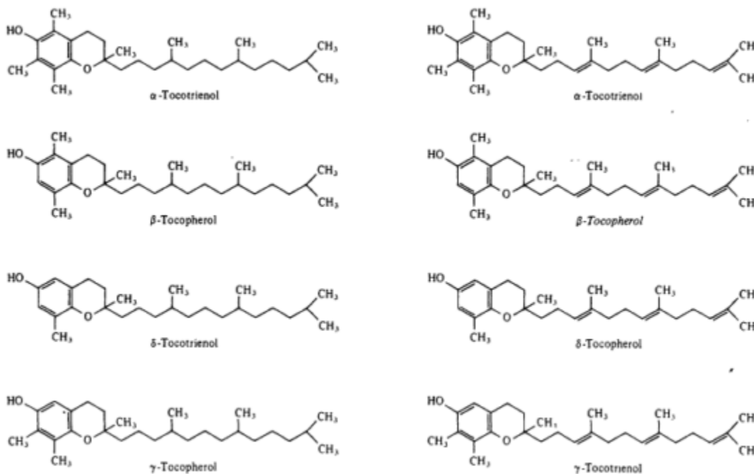
Figure 7 Chemical structures of naturally occurring vitamin E-active compounds and analogues.
