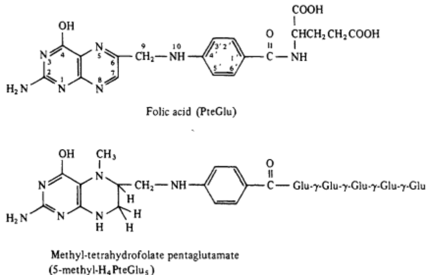
Figure 14 Chemical structures of folic acid and 5-methyltetrahydrofolate.
