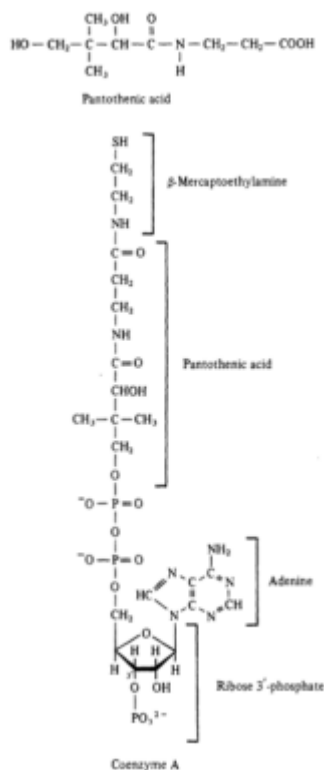
Figure 15 Chemical structures of pantothenic acid and coenzyme A.
