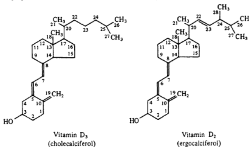
Figure 2 Chemical structures of vitamin D 3 and vitamin D 2 .
