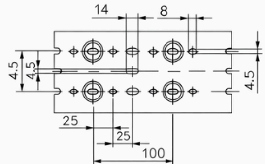
MOUNTING HOLE PATTERN Width: 25mm only Wide & Thin Finger
