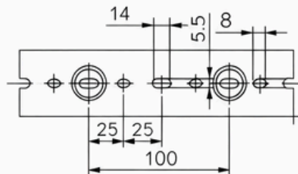
MOUNTING HOLE PATTERN Width: 40 & 60 mm Wide & Thin Finger
