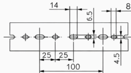
MOUNTING HOLE PATTERN Width: 25mm only Wide & Thin Finger
