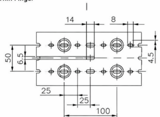
MOUNTING HOLE PATTERN
