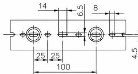
MOUNTING HOLE PATTERN
