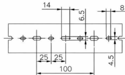
MOUNTING HOLE PATTERN
