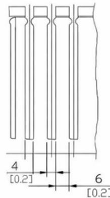
Finger Dimensions
