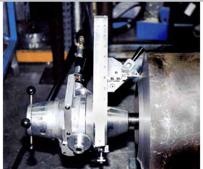
The versatile Model 214B BEVELMASTER with Single Point module generating a precision compound bevel on heavy wall pipe.
