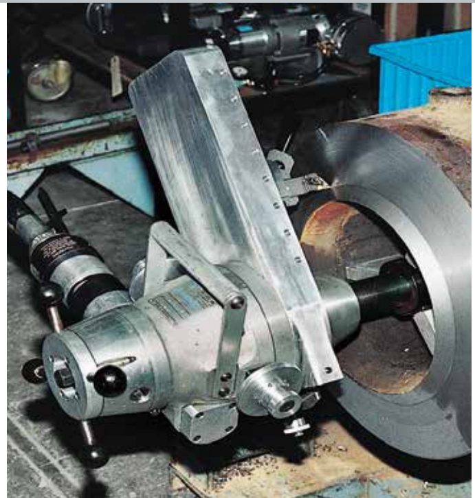
Tri Tool's popular BEVELMASTER Model 214B has been configured with a single point machining module to produce this precision compound bevel on a very heavy wall, flame-cut header pipe.
