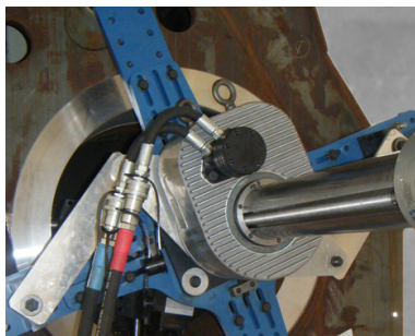
BB7100 Boring Machine
