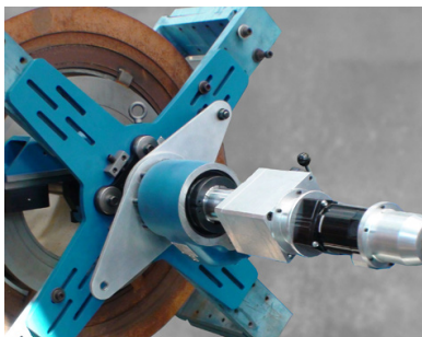
BB6100 Boring Machine
