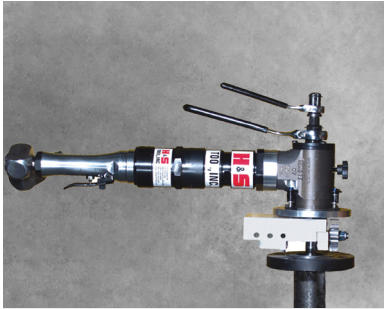
MODEL BF Flange Facer
