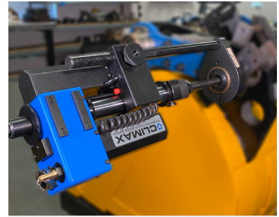
BW3000 Auto Bore Welder
