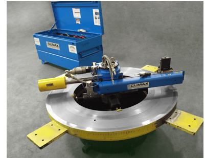
FF6300 Flange Facer
