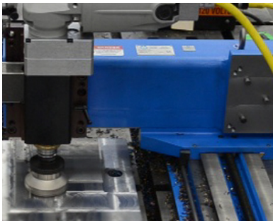
PM4200 Milling Machine
