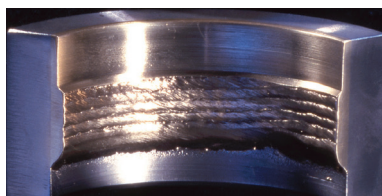
Aluminum bronze bore weld
