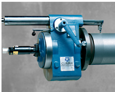
PL3000 Lathe
