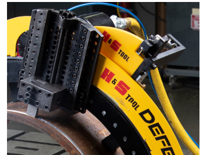
BFC Split-Frame Machine
