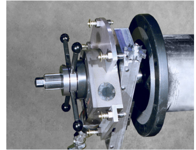
MODEL MTF Flange Facer
