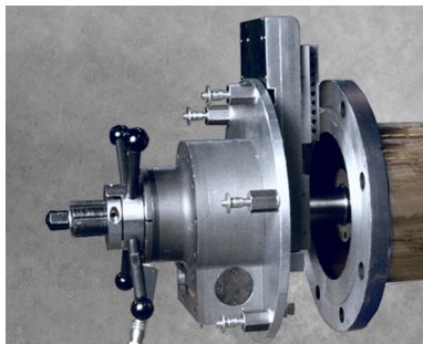
MODEL MFTF Flange Facer
