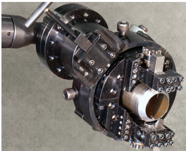
MFC Split-Frame Machine
