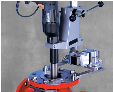
VM2000 Globe Valve Seat Grinding and Safety Valve Repair
