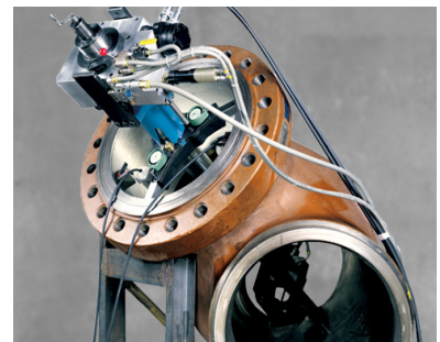
VM9000 Valve Repair System*
