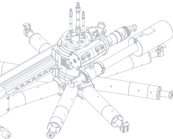
FLANGE FACERS
