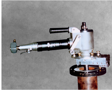
MODEL MSF Flange Facer
