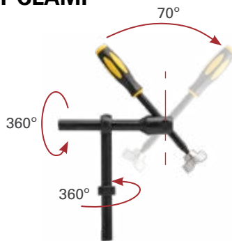
Angled Clamping
