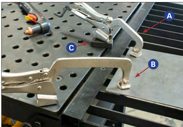
Insert the Inserta Pliers into the 5/8" holes on the Rhino Cart® Tabletop.
