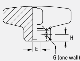
Reamed Thru
