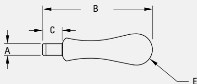
Solid Handle - Threaded Shank
