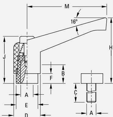
Tapped Type
