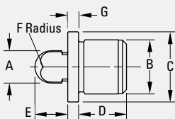
Relieved
