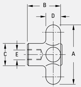
Tapped Type
