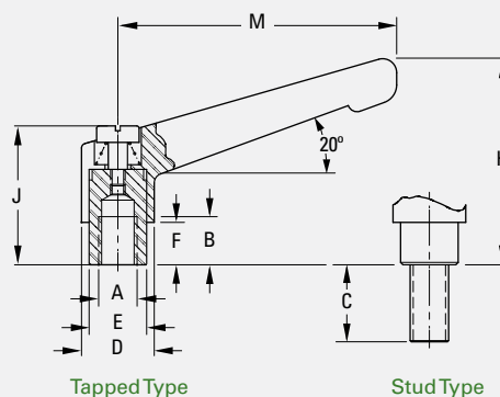
Tapped Type
