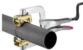
Pipe Pliers The Easy Way to butt-weld pipes
