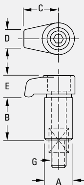
Socket Head Cap Screw Style
