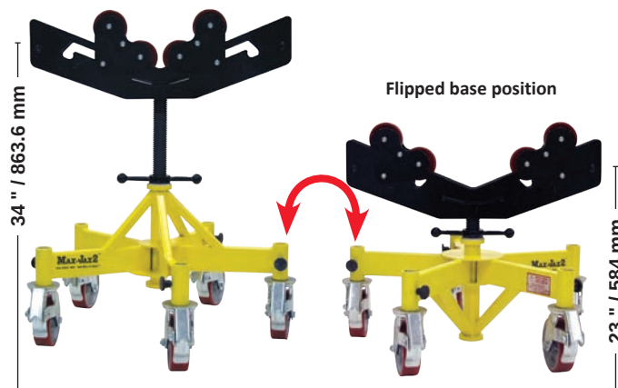
Lo Max Jax™ 2 Kit with rocking steel wheels in V-head and casters PART NO 3310RSWH
