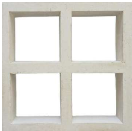
Chemax 50x50x10cm - 7kg 4pz/m 2
