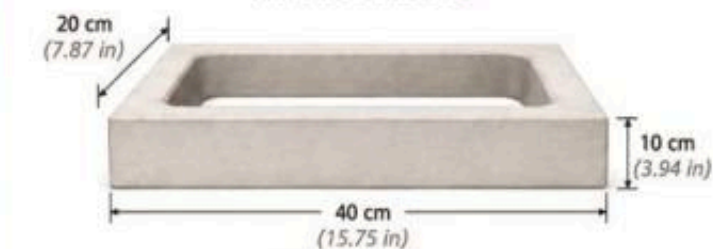
PERSPECTIVA HORIZONTAL HORIZONTAL PERSPECTIVE
