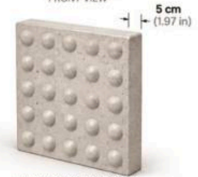
PERSPECTIVA VERTICAL VERTICAL PERSPECTIVE
