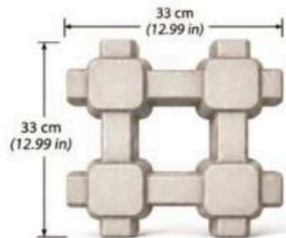
VISTA FRONTAL FRONT VIEW
