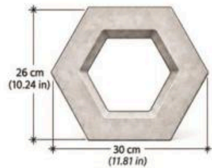
VISTA FRONTAL FRONT VIEW
