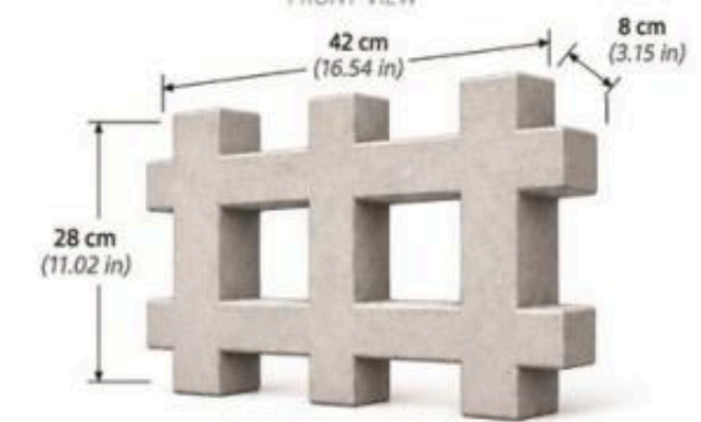
PERSPECTIVA VERTICAL VERTICAL PERSPECTIVE
