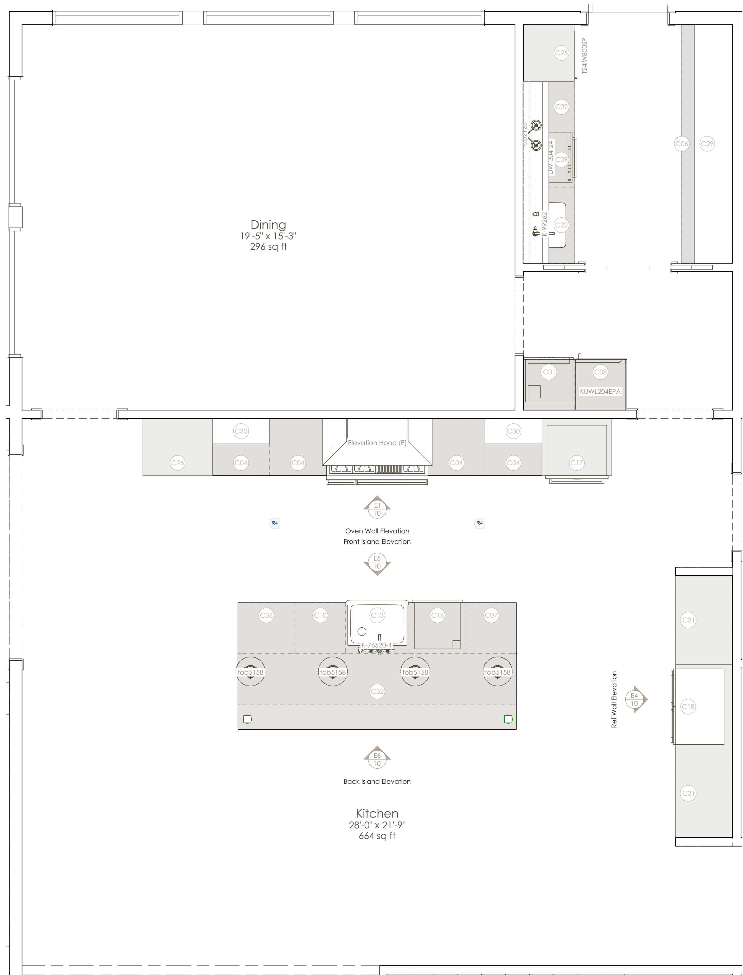
KITCHEN AND BATH PLAN VIEW 1/2 IN = 1 FT
