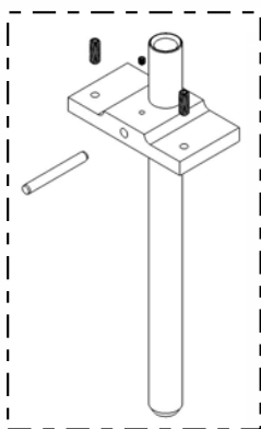
34634 ASSY
