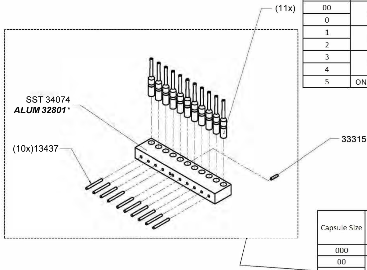
Complete Assembly
